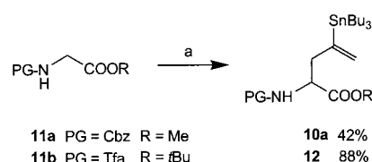
Scheme 8. a) 1) 2.5 equiv LDA, 1.1 equiv ZnCl 2 , THF, −78 °C; 2) 0.8 equiv 9b , 1% [allyl]PdCl 2 , 4.5% PPh 3 , −78 °C → RT.
