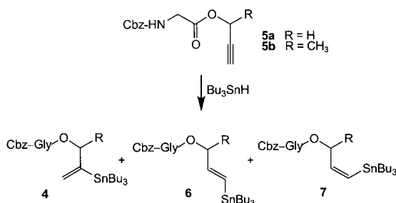
Scheme 5. Hydrostannylation of propargylic esters.
