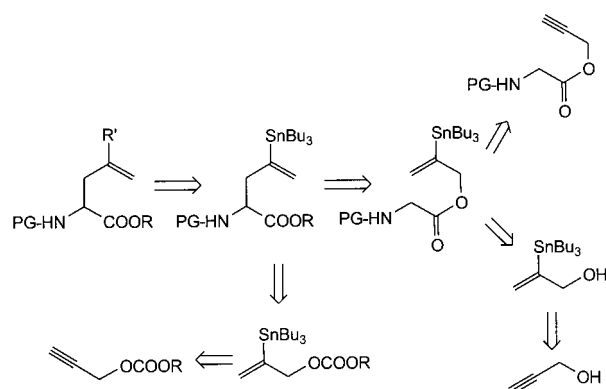
Scheme 3. Retrosynthetic approach.
