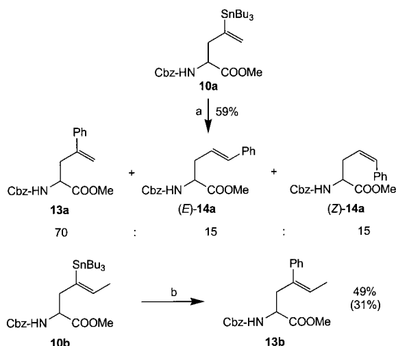
Scheme 9. a) 3 equiv PhBr, 2.5 mol % [\text{Pd}_2(\text{dba})_3] \cdot \text{CHCl}_3 , 20 mol % \text{AsPh}_3 , THF, 65 °C, 20 h (59 %). b) 3 equiv PhBr, 2.5 mol % [\text{Pd}_2(\text{dba})_3] \cdot \text{CHCl}_3 , 20 mol % \text{AsPh}_3 , toluene, 90 °C, 20 h.
