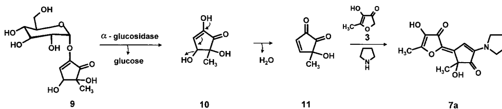
Scheme 5. Generation of 2,4,5-Trihydroxy-5-methylcyclopent-2-en-1-one ( 10 ) by \alpha -Glucosidase Treatment of 2-( \alpha -D-Glucopyranosyloxy)-4,5-dihydroxy-5-methylcyclopent-2-en-1-one ( 9 ) and Formation of Chromophore 7a,b via 5-Hydroxy-5-methylcyclopent-3-ene-1,2-dione ( 11 ) as a Key Intermediate
