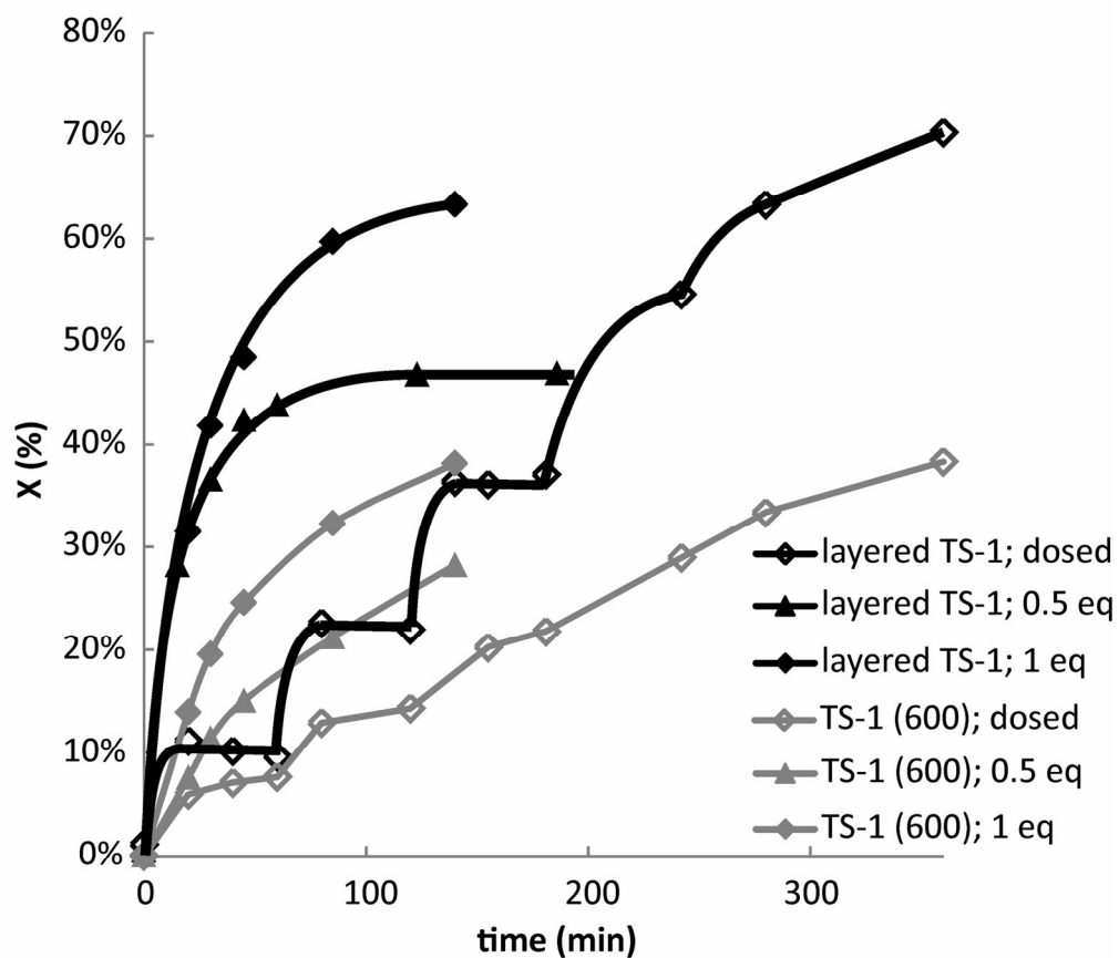
Figure 9: Development of conversion in time using different amount of H 2 O 2 and dosing of the oxidant over TS-1 (600) (gray) and layered TS-1 (black). 74x66mm (600 x 600 DPI)
