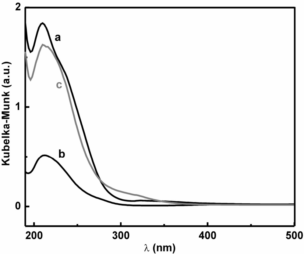
Figure 4: DR-UV-Vis spectra of the Ti-UTL (a), Ti-IPC-1-PI (b) and Ti-IPC-2 (c). 70x60mm (600 x 600 DPI)
