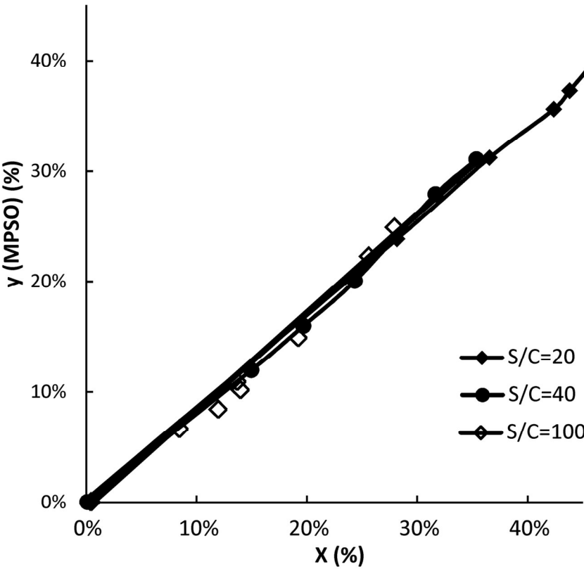
Figure 8: Selectivity curves of MPS oxidation over layered TS-1 using different S/C ratio. 68x57mm (600 x 600 DPI)
