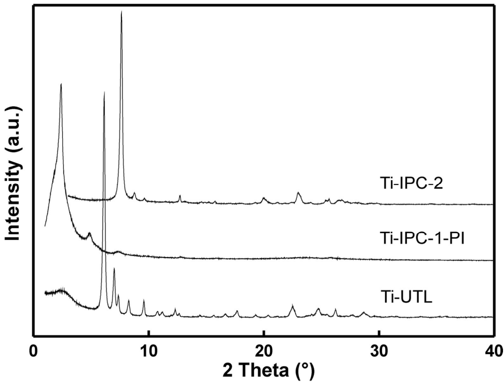
Figure 2: Powder XRD patterns of the UTL based catalysts. 64x50mm (600 x 600 DPI)
