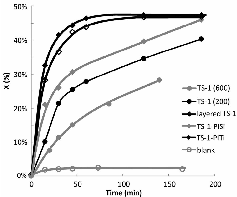
Figure 5: Catalytic oxidation of methylphenyl sulphide (MPS) over the TS-1 based catalysts at 30°C. Reaction conditions: 8 mmol of MPS, 4 mmol of H 2 O 2 (35 wt.%) , 50 mg of catalyst, 250 µl of internal standard, 10 ml acetonitrile, 900 rpm. 69x57mm (600 x 600 DPI)
