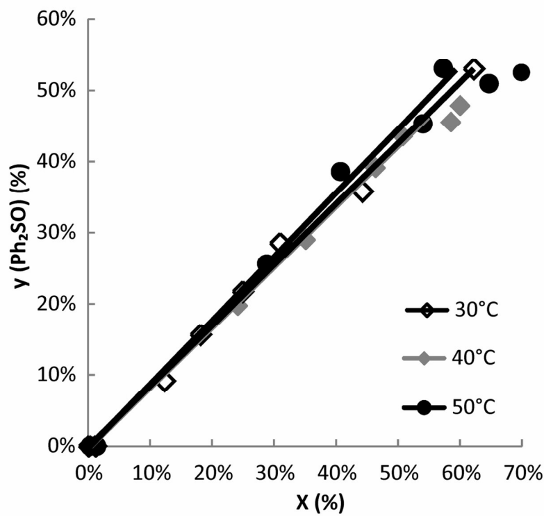
Figure 12: Selectivity curves for Ph 2 SO in oxidation of Ph 2 S over TS-1-PITi at different temperature. 63x48mm (600 x 600 DPI)
