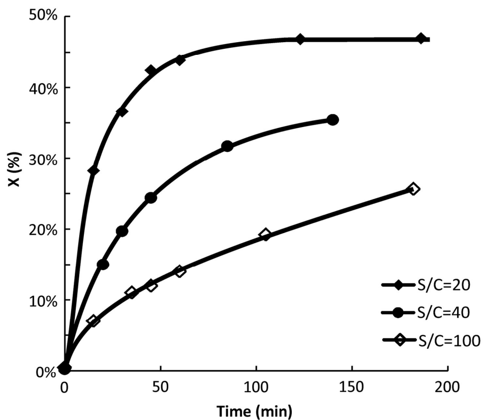
Figure 7: Conversion curves of MPS oxidation over layered TS-1 using different S/C ratio. 69x57mm (600 x 600 DPI)
