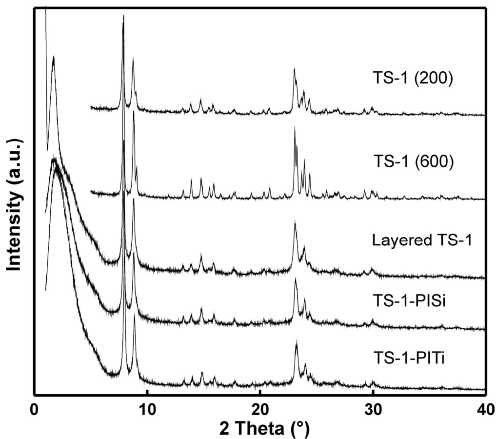
Figure 1: Powder XRD patterns of the TS-1 based catalysts. 74x68mm (600 x 600 DPI)
