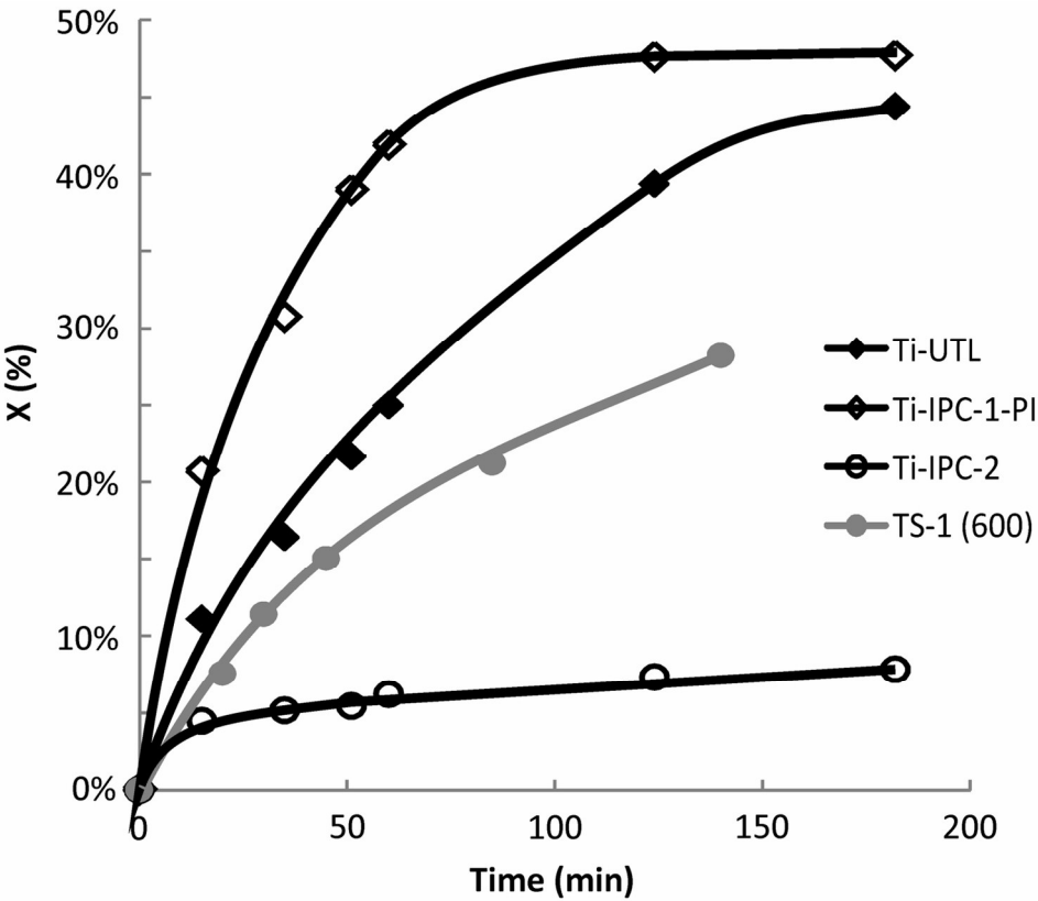
Figure 6: Catalytic oxidation of methylphenyl sulphide (MPS) over the Ti-UTL based catalysts at 30°C. TS-1 (600) is shown as a benchmark. Reaction conditions: 8 mmol of MPS, 4 mmol of H 2 O 2 (35 wt.%) , 50 mg of catalyst, 250 µl of internal standard, 10 ml acetonitrile, 900 rpm. 68x56mm (600 x 600 DPI)
