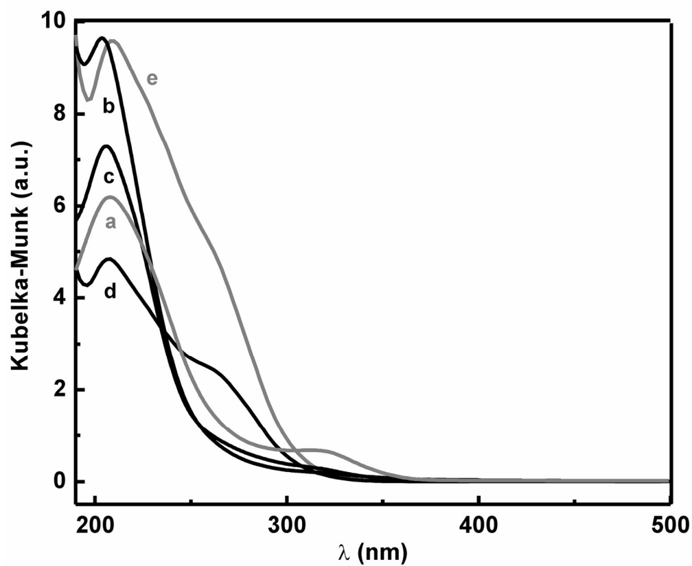
Figure 3: DR-UV-Vis spectra of the TS-1 (200) (a), TS-1 (600) (b), layered TS-1 (c), TS-1-PISi (d), TS-1-PITi (e). 69x57mm (600 x 600 DPI)
