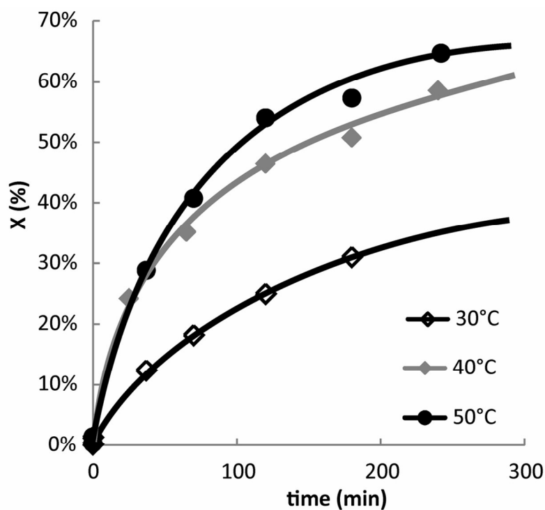
Figure 11: Conversion curves of oxidation of Ph 2 S over TS-1-PITi at different temperatures. 60x44mm (600 x 600 DPI)
