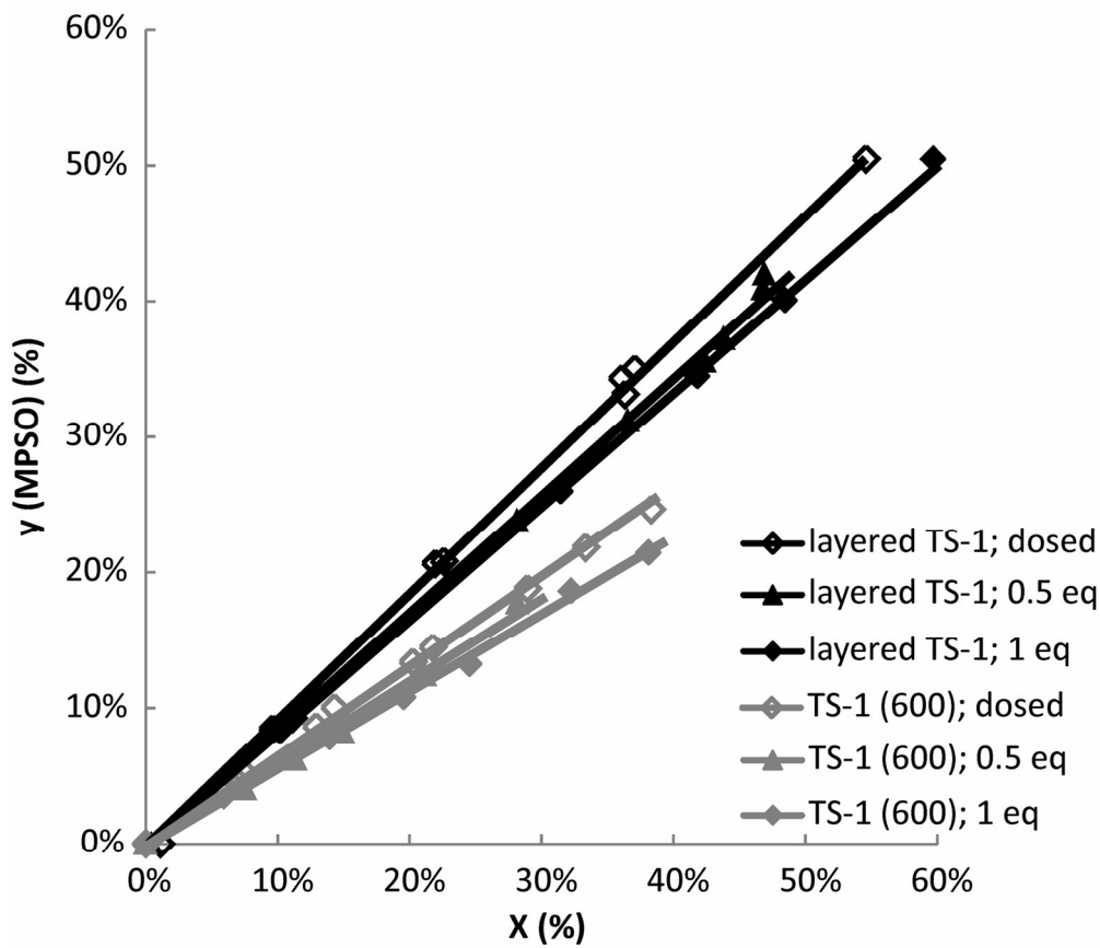
Figure 10: Selectivity curves of the experiments using different amount of H 2 O 2 and dosing of the oxidant over TS-1 (600) (gray) and layered TS-1 (black). 72x62mm (600 x 600 DPI)
