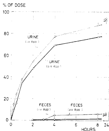
Figure 1.—Excreted fractions of radioactivity in the feces after administration of pyrovalerone-HCl to the mouse (i.v.: 10 mg/kg; orally: 20 mg/kg). 5
