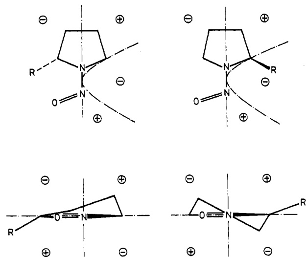
Figure 8. Projections of equatorial Z and E conformers of N -nitrosopyrrolidine substituted at C-2.
