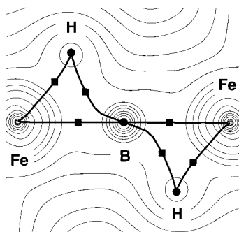
Figure 4. Contour lines of the charge density (thin) and the molecular graph (bold) in the bridging region of 1 . Bond critical points are denoted by squares (■).
