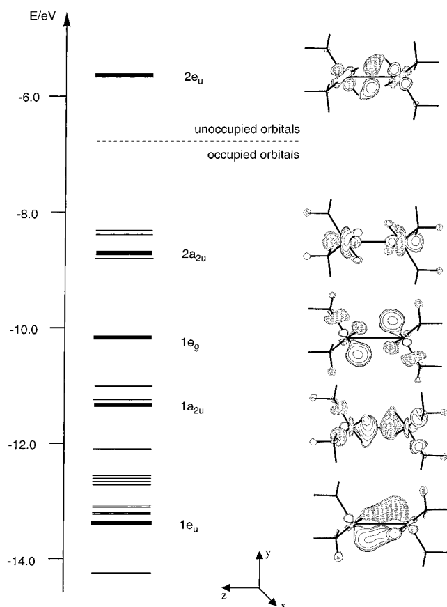
Figure 3. Orbital energy levels for 1 , labeled according to D_{3d} symmetry. Selected orbitals are also depicted, for which the corresponding energy lines appear in bold.
