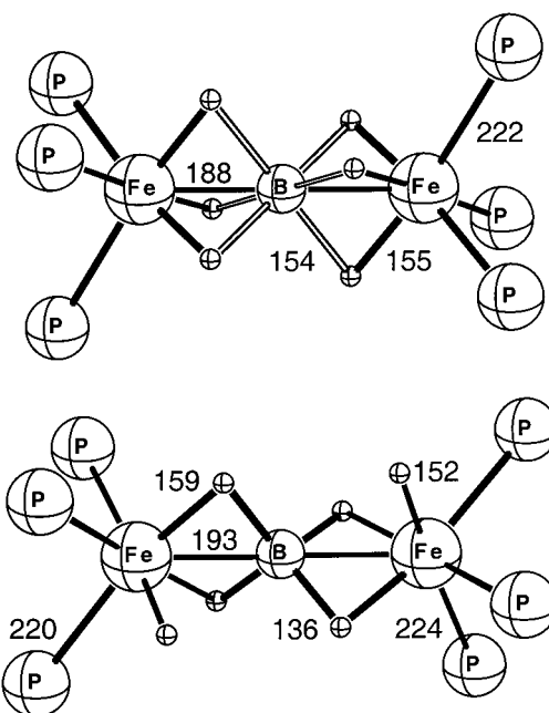
Figure 2. Optimized BP86 geometries and selected bond distances (in pm) for the [\{\text{Fe}(\text{PH}_3)(\text{H})_3\}_2\text{B}]^+ model compounds I (above) and II (below) ( \text{P} = \text{PH}_3 ).
