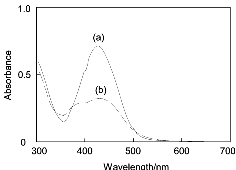
Figure 1. UV-vis spectra of trans - 1 in toluene (a) before irradiation and (b) after irradiation at 420 nm from a cutoff-filtered xenon lamp for 1 h at 20 °C (photostationary state).
