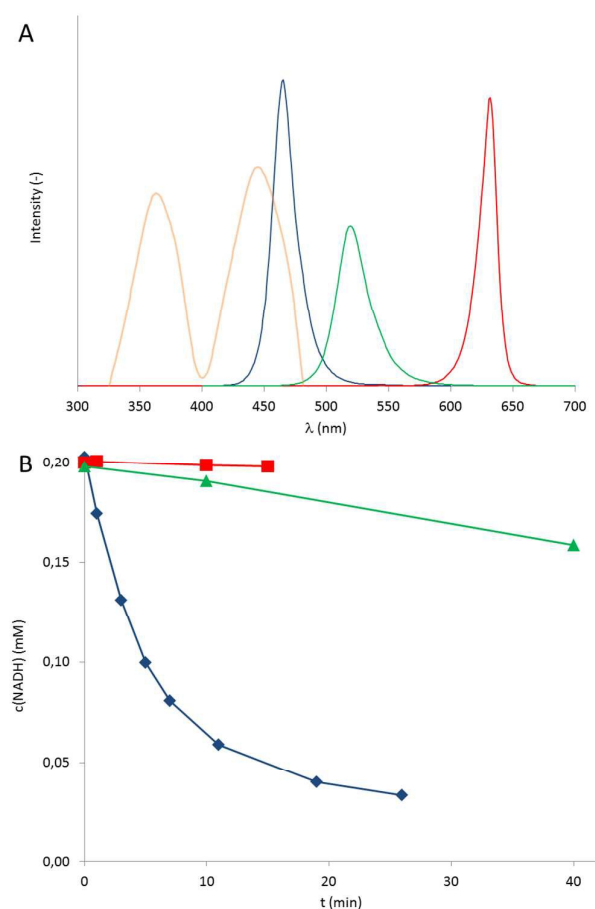
Figure 1. Emission wavelengths of the LEDs used (A) and the influence of the LED wavelength on the rate of the photocatalytic aerobic NADH oxidation (B). A: the emission spectra of the blue, green and red LED are shown (in arbitrary units) together with the absorption spectrum of the FMN photocatalyst, yellow). B: Time course of the aerobic oxidation of NADH catalysed by FMN and red (●), green (▲) or blue (◆) light. Conditions: 50 mM KPi Buffer (pH 7), [\text{NADH}]_0 = 0.2 \text{ mM} , [\text{FMN}] = 2 \mu\text{M} , T = 30^\circ\text{C} .
