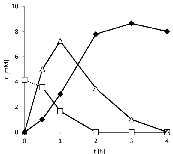
Figure 3. Time course of the photoenzymatic oxidation of meso -3-methyl-1,5-pentanediol (□) to ( S )-4-methyltetrahydro-2H-pyran-2-one (◆) via the intermediate lactol (△). General conditions: 100 mM Glycine-NaOH buffer (pH 9), 100 mM. [diol] 0 = 10 mM, [NADH] 0 = 1 mM, [FMN] = 100 μM, [HLADH] = 7.4 μM, 5 drops of catalase, T = 30°C.
