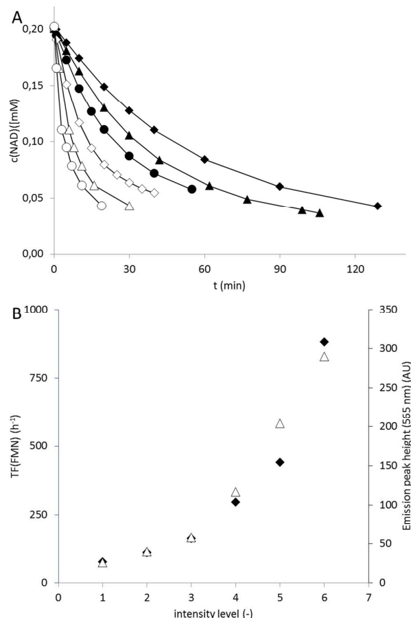
Figure 2. A: Influence of the intensity of the Blue LED in the oxidation of NADH in presence of FMN. Conditions: 50 mM KPi Buffer (pH 7), T = 30^\circ\text{C} , [\text{NADH}]_0 = 0.2 \text{ mM} , [\text{FMN}] = 2 \mu\text{M} ; relative blue light intensity :1:◆, 2:▲, 3:●, 4:◇, 5:△, 6:○; B: Dependence of the rate of the FMN-catalysed NADH oxidation (expressed as TF of the FMN catalyst, ◆) on the intensity of the blue LED (▲). Conditions: KPi Buffer (pH 7, 50 mM), T = 30^\circ\text{C} , [\text{NADH}]_0 = 0.2 \text{ mM} , [\text{FMN}]_0 = 2 \mu\text{M}
