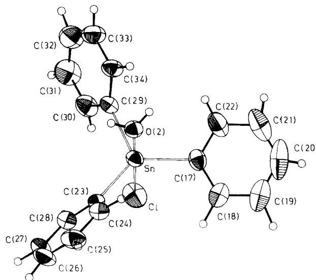
Fig. 2. ORTEP diagram of [\text{SnPh}_3\text{Cl}(\text{OH}_2)] in compound 2 . Thermal ellipsoids are drawn at the 40% probability level.
