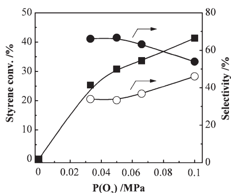
Figure 2. Effect of \text{O}_2 pressure on catalytic performances for epoxidation of styrene over \text{Fe}_3\text{O}_4 . The other reaction conditions are the same as in Figure 1. (●) styrene oxide, (○) benzaldehyde.
