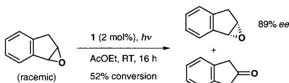
Scheme 1. Kinetic resolution of (±)-indene oxide.
