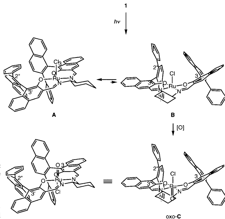
Scheme 4. Proposed structures of the photoactivated [Ru(salen)] and the oxo(salen)ruthenium species.
