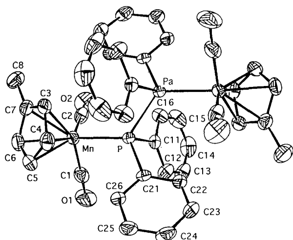
Fig. 1. ORTEP drawing of [(\text{MeCp})\text{Mn}(\text{CO})_2]_2(\mu\text{-Ph}_2\text{PPPh}_2) . Only one half of the molecule is labelled because of the presence of an inversion centre. The Pa and P atoms are related by the inversion centre. Thermal ellipsoids are drawn with 30% probability boundaries.
