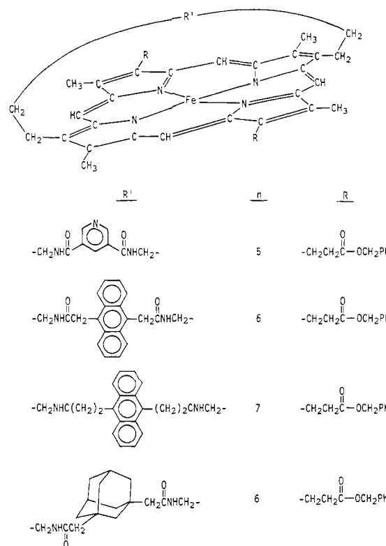
Figure 1. Cyclophane heme compounds.
