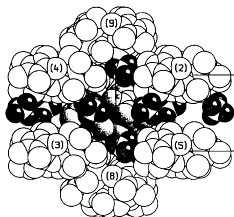
Figure 3. Space-filling model of the pseudohexagonal close-packing ( ABABA ) in 1b ; molecules in the plane of the reference molecule (RM) have been omitted for clarity. (shaded spheres: reference molecule (RM); black spheres: fluorine atoms of the \text{BF}_4 groups; open spheres: environment molecules).
