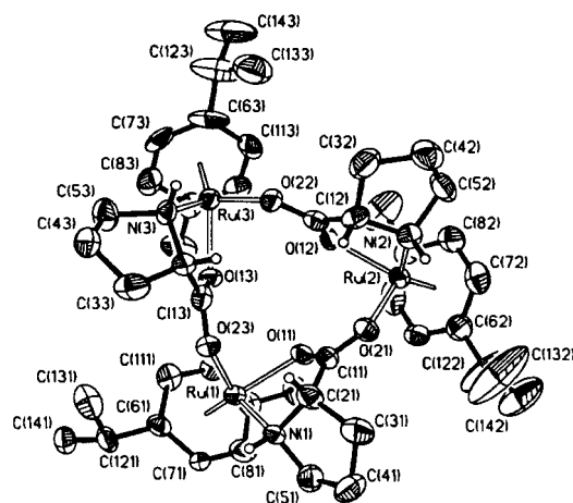
Figure 2. View of the trinuclear cation of 6c with the atom numbering scheme. Only hydrogen atoms bonded to the two asymmetric atoms of each proline ring have been included in the drawing for clarity.
