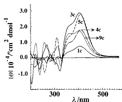
Figure 14. CD spectra of the ruthenium trimers [(\eta^6\text{-}p\text{-MeC}_6\text{H}_4i\text{Pr})\text{Ru}(\text{Ala})]_3(\text{BF}_4)_3 \cdot \text{H}_2\text{O} ( 1c ), [(\eta^6\text{-}p\text{-MeC}_6\text{H}_4i\text{Pr})\text{Ru}(\text{Val})]_3(\text{BF}_4)_3 \cdot \text{H}_2\text{O} ( 3c ), [(\eta^6\text{-}p\text{-MeC}_6\text{H}_4i\text{Pr})\text{Ru}(\text{Tle})]_3(\text{BF}_4)_3 \cdot \text{H}_2\text{O} ( 4c ), [(\eta^6\text{-}p\text{-MeC}_6\text{H}_4i\text{Pr})\text{Ru}(\text{Phe})]_3(\text{BF}_4)_3 \cdot \text{H}_2\text{O} ( 5c ), and [(\eta^6\text{-}p\text{-MeC}_6\text{H}_4i\text{Pr})\text{Ru}(\text{Hyp})]_3(\text{BF}_4)_3 \cdot \text{H}_2\text{O} ( 9c ) in acetone.
