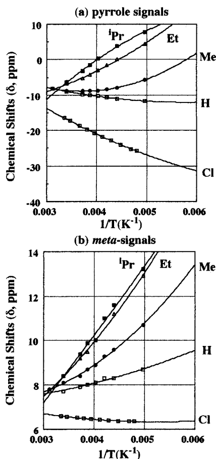
Figure 2. Curie plots of the pyrrole (a) and meta -proton (b) signals of [\text{Fe}(\text{TPP})(\text{CN})_2]^- , [\text{Fe}(\text{R-TPP})(\text{CN})_2]^- (R = Me, Et, i\text{Pr} ), and [\text{Fe}(\text{Cl-TPP})(\text{CN})_2]^- taken in \text{CD}_2\text{Cl}_2 – \text{CD}_3\text{OD} solution.
