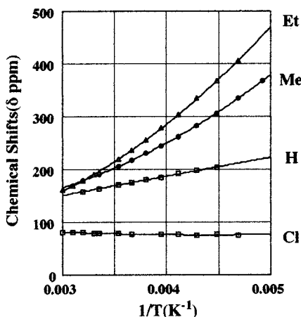
Figure 3. Curie plots of the meso -carbon signals of [\text{Fe}(\text{TPP})(\text{CN})_2]^- , [\text{Fe}(\text{R-TPP})(\text{CN})_2]^- (R = Me, Et, i\text{Pr} ), and [\text{Fe}(\text{Cl-TPP})(\text{CN})_2]^- taken in \text{CD}_2\text{Cl}_2 – \text{CD}_3\text{OD} solution.
