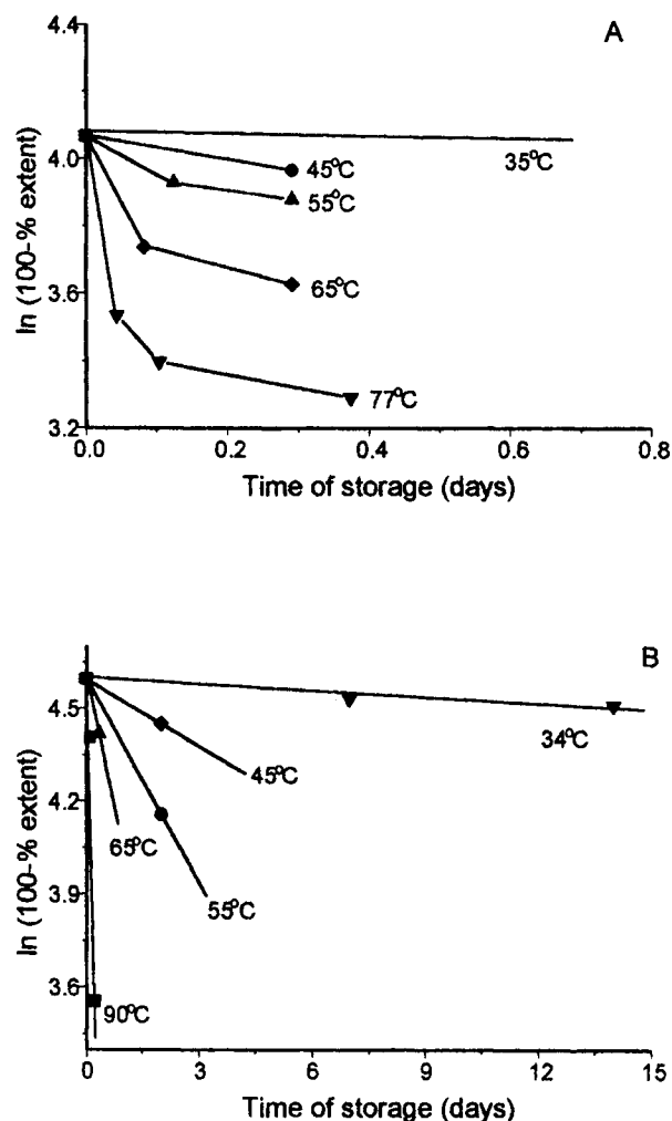
Fig. 3. Kinetic treatment of data from Figure 2, assuming first-order kinetics for (A) Physalaemin and (B) Hamburger peptide.
