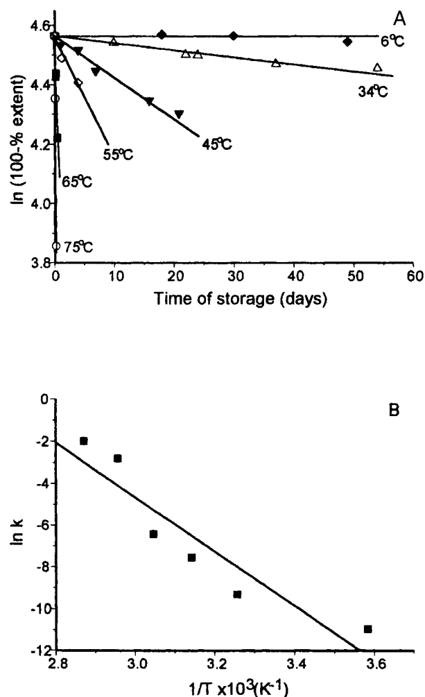
Fig. 5. (A) Kinetic treatment of spectrophotometric data for the hydrolysis of npTHP in Ficoll (MW 400,000), T_g = 45^\circ C , water content 4.3% and (B) the Arrhenius plot.
