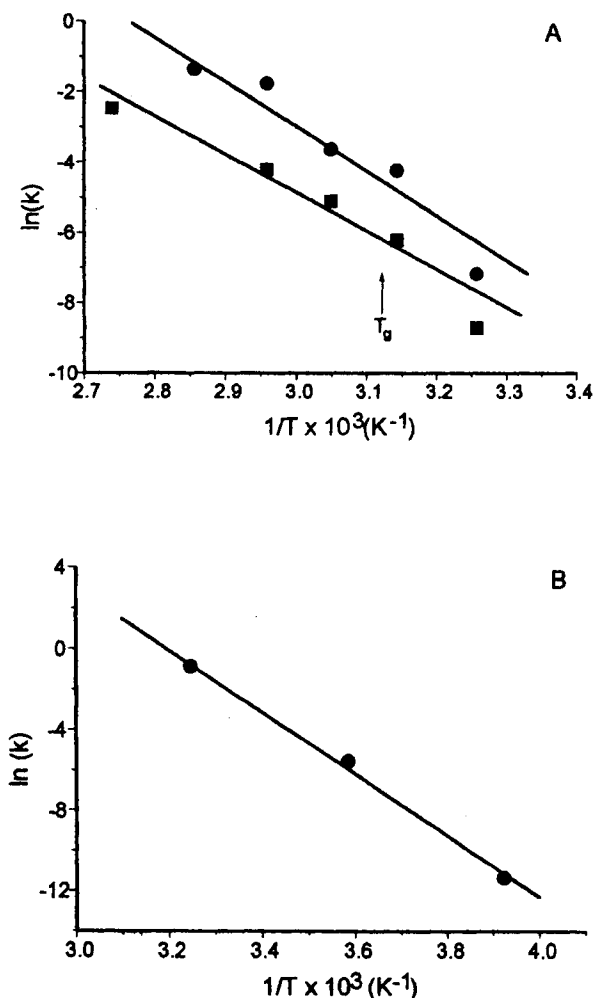
Fig. 4. Arrhenius plots for (A) the hydrolysis of Asp-Pro in Physalae-min (●) and Hamburger (■) peptide and for (B) the hydrolysis of npTHP in 10% (w/w) aqueous solutions of sucrose and Ficoll HMW (data points, taken from Table III, overlap within the experimental error).
