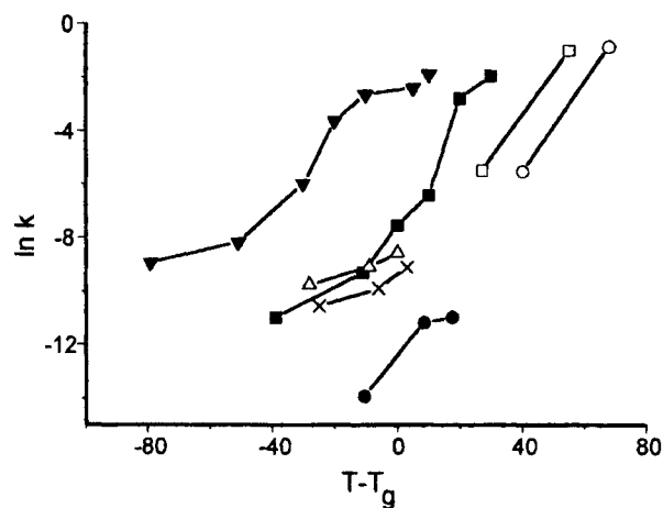
Fig. 6. Temperature dependence of the hydrolysis rate of npTHP with T_g as the reference temperature in freeze-dried 10% (w/w) aqueous formulations of Dextran ( \blacktriangledown ), Ficoll, HMW, 400,000 MW ( \blacksquare ), Ficoll, LMW, 70,000 MW ( \times ), Byco A ( \triangle ) and sucrose ( \bullet ) and in freeze-concentrated formulations of Ficoll, HMW ( \square ) and sucrose ( \circ ) (with T_g' as reference temperature).
