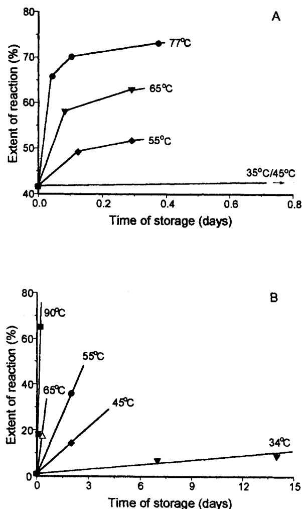
Fig. 2. Extent of release of Pro as a function of storage time for (A) Physalaemin (Ficoll, 400K, T_g = 49^\circ\text{C} , water content 2.2%) and (B) Hamburger peptide (Ficoll, 400K, T_g = 46^\circ\text{C} , water content 4.0%).
