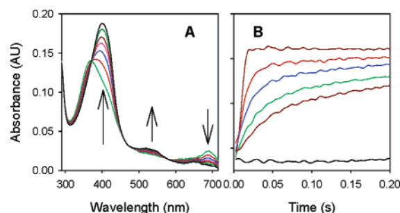
Figure 1. (A) Time-resolved UV–vis spectrum for reaction of CPO Compound I with 0.10 mM styrene over 330 ms. (B) Kinetic traces at 400 nm for reactions of CPO Compound I with styrene at (from the bottom) 0, 0.10, 0.20, 0.40, 0.8, and 1.6 mM concentrations.
