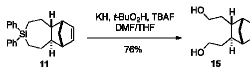
Scheme 3. Fleming-Tamao Oxidation
