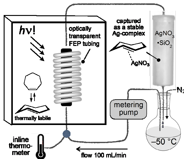
Figure 1 The apparatus for photoisomerization of carbocyclic trans -cycloheptene derivatives was designed to minimize loss of trans -cycloheptene due to thermal isomerization by using FEP tubing and inline cooling. For the synthesis of trans -1-sila-4-cycloheptenes, photoisomerizations could be carried out at rt using a conventional flow photoisomerization setup.
