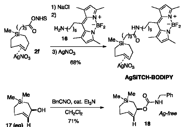
Scheme 4. Transformations of Si-TCH derivatives
