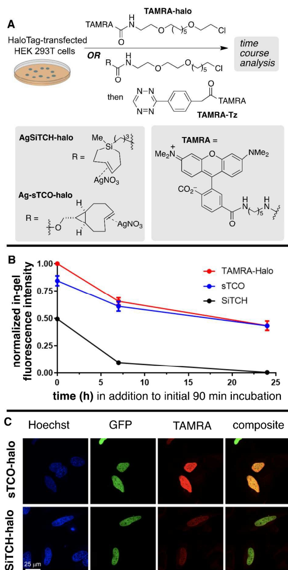
Scheme 9. Live cell stability and imaging studies of SiTCH-Halo. (A) In the stability experiment, HEK293T cells expressing HaloTag were treated with 10 \mu M Ag-sTCO-Halo or AgSiTCH-Halo for 30 min, followed by two 30 min wash periods. Control cells were treated with 2 \mu M TAMRA-Halo . At 0, 7, and 24 h time points, 2 \mu M TAMRA-Tz was added and allowed to react for 1 h before analysis. (B) Cellular stability of Ag-sTCO-Halo and AgSiTCH-Halo . In-gel fluorescent intensities were normalized by the corresponding Western blot signals, and were subsequently normalized by the value of TAMRA-Halo at time 0. Data were plotted as mean \pm SEM. (C) Live cell images of HeLa cells expressing Halo-H2B-GFP. Cells were labeled with 10 \mu M Ag-sTCO-Halo or AgSiTCH-Halo for 30 min, followed by two 30 min wash periods, before the treatment with 1 \mu M TAMRA-Tz for 5 min. The reactions were quenched with 100 \mu M TCO-amine for 10 min, followed by two 30 min wash periods prior to addition of 8 \mu M Hoechst 33342 to visualize the nuclei and confocal imaging. Signals of Hoechst, GFP, and TAMRA were shown in blue, green, and red, respectively. Colocalization was demonstrated in composite images of GFP and TAMRA. Scale bar = 25 \mu m.
