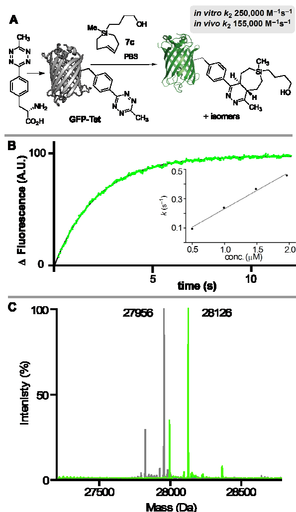
Scheme 7. (A) GFP-Tet reacts with 7c to give a Diels-Alder adduct. Because the tetrazine quenches GFP fluorescence, the reaction progress can be measured by monitoring fluorescence increase. (B) Stopped-flow kinetic data for the reaction of GFP-Tet (50 nM) with 7c (1.96 \mu\text{M} ) at 25^\circ\text{C} in PBS with fluorescence monitoring (Ex: 488 nm; Em: 506 nm). Data points are shown in green, and the fit is shown in black. A second order rate constant ( k_2 ) was determined by plotting k_{\text{obs}} vs. the concentration of Si-TCH 7c . (C) Quantitative determination of the cycloadduct was confirmed by ESI-MS. Deconvoluted Mass spectra of GFP-Tet (grey) and the cycloadduct (green) are displayed and show the expected mass shift of 170 Da. Smaller peaks in each spectrum correspond to proteins that are truncated by a methionine.
