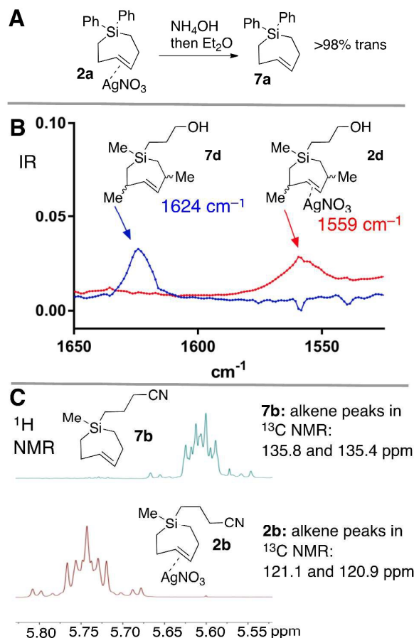
Figure 3 (a) Decomplexation of AgNO 3 with NH 4 OH gives metal-free Si-TCH 7a which is stable to overnight storage in solution. Aq. NaCl can also be used to liberate metal from SiTCH•AgNO 3 complexes. The metal-free complexes are stable in solution, but give variable amounts of isomerization when concentrated to dryness. (b) FT-IR spectrum of the C=C stretches of metal complex 2d and free alkene 7d . (c) Diagnostic shifts in alkene peaks in the 1 H and 13 C NMR spectra of metal complex 2b and metal-free 7b .
