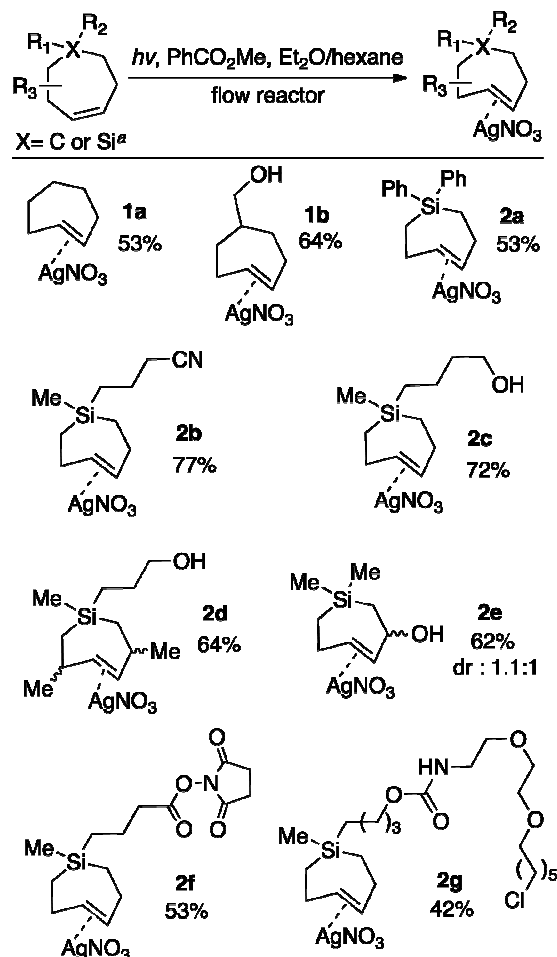
Scheme 1. Flow-photochemical synthesis of AgNO 3 complexes of trans -cycloheptenes and trans -1-sila-4-cycloheptenes.
