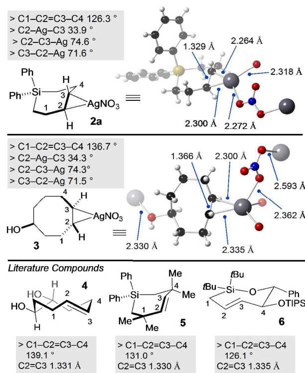
Figure 2 X-ray crystal structures of SiTCH•AgNO 3 and TCO•AgNO 3 complexes, with comparisons to known metal-free trans -cycloalkenes that have been crystallographically characterized.
