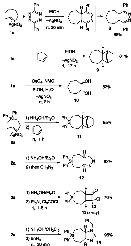
Scheme 2. Reactions of TCH 1a and Si-TCH 2a .
