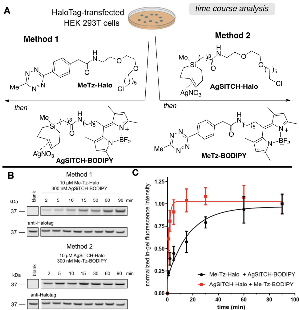
Scheme 8. Reactions of AgSiTCH with 3-methyl-6-s-tetrazine derivatives in live HEK 293T cells expressing HaloTag. (A) Cells were treated with 10 \mu M MeTz-Halo (method 1) or AgSiTCH-Halo (method 2) for 30 min, followed by two 30 min washings and treatment with 300 nM AgSiTCH-BODIPY (method 1) or 300 nM MeTz-BODIPY (method 2) for the indicated time. (B) Analyzed by in-gel fluorescence and Western blot for each method: in-gel fluorescence is shown on the top panel, and Western blot with an anti-HaloTag antibody is on the bottom panel. (C) Time course for the two reactions in B. In-gel fluorescence intensity from n = 3 independent replicates was normalized by the corresponding Western blot signal, and was fit to a one-phase exponential equation. Data were plotted as mean \pm SEM.
