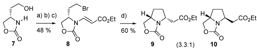
Scheme 2. (a) p -TsCl, pyridine, DCM; (b) \text{HCCCCO}_2\text{Et} , NMM, DCM, reflux; (c) LiBr, acetone, reflux; (d) 1.3 equiv. \text{Bu}_3\text{SnH} , 0.15 equiv. AIBN, benzene (0.025 M), reflux, 5 h (syringe pump, 4 h)
