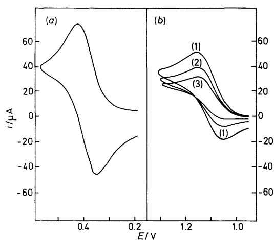
Figure 6. (a) Cyclic voltammetry of [Fe(bzimpy) 2 ][ClO 4 ] 2 vs. the non-aqueous Ag + /Ag reference electrode in CH 3 CN-[NEt 4 ][ClO 4 ]; scan rate 100 mV s -1 . (b) Cyclic voltammetry of [Fe(bztpy) 2 ][ClO 4 ] 2 in CH 3 NO 2 -[NEt 4 ][ClO 4 ]; scan rates, (1) 400, (2) 200, (3) 100 mV s -1 ; current ratio ( i_{p,c}/i_{p,a} ), (1) 0.798, (2) 0.689, (3) 0.550
