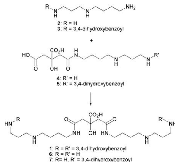
Scheme 1 Possible reactions catalysed by AsbB in petrobactin 1 biosynthesis.
