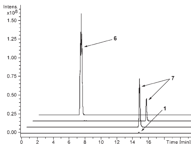
Fig. 1 Extracted ion chromatograms from LC-MS analyses, in positive ion mode, of incubations of AsbB, ATP, and \text{Mg}^{2+} with 4 and 2 (top trace, m/z 447.3), 4 and 3 (second trace, m/z 583.3), 5 and 2 (third trace, m/z 583.3), and 5 and 3 (bottom trace, m/z 719.3).
