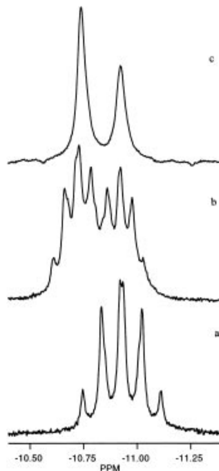
Figure 1. (a) Partial ^1\text{H} NMR spectrum (hydride region) of complex 1 (300 MHz, 298 K) in acetone- d_6 and (b) after exposure to \text{D}_2 (1 atm) for 11 h (500 MHz). (c) ^1\text{H}\{^{31}\text{P}\} spectrum (500 MHz).
