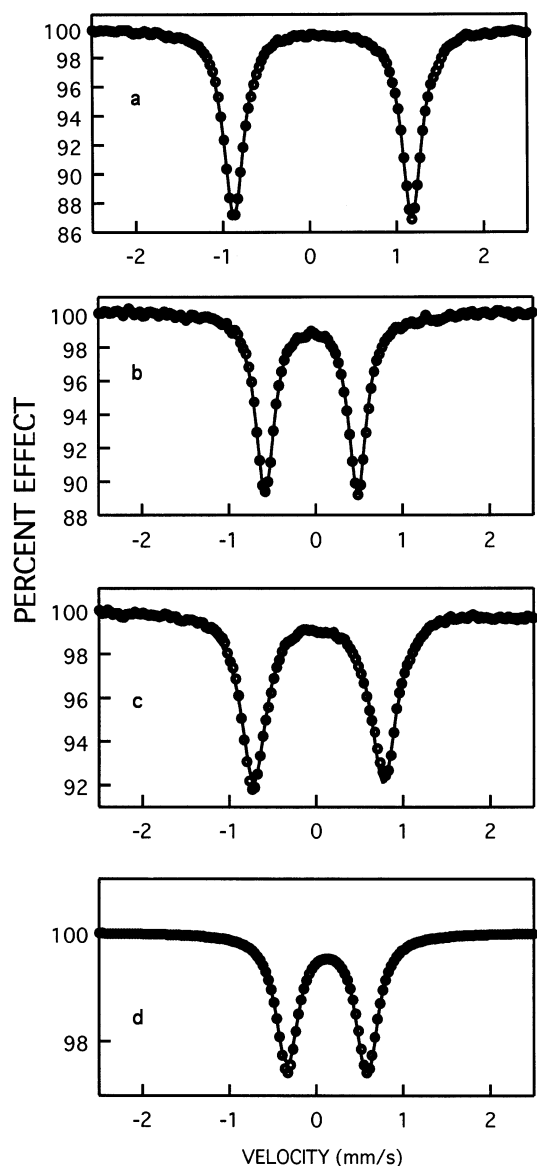
Fig. 1. Selected Mössbauer spectra at 80 K of (a) \text{Cp}^*(\text{dppe})\text{Fe}-\text{C}\equiv\text{C}-\text{H} ( 4a ); (b) [\text{Cp}^*(\text{dppe})\text{Fe}-\text{C}\equiv\text{C}(\text{Ph})\text{H}][\text{PF}_6] ( 6a ); (c) [\text{Cp}^*(\text{dppe})\text{Fe}-\text{C}\equiv\text{C}-\text{C}\equiv\text{C}(\text{OMe})][\text{BPh}_4] ( 7 ); (d) [\text{Cp}^*(\text{dppe})\text{Fe}-\text{C}\equiv\text{C}-\text{Ph}][\text{PF}_6] ( 4b +).
