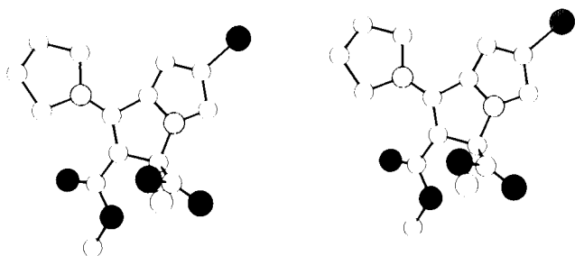
Figure 1. A stereodrawing of molecule III. The non-carbon as follows: Br - ; N - ; O - .
