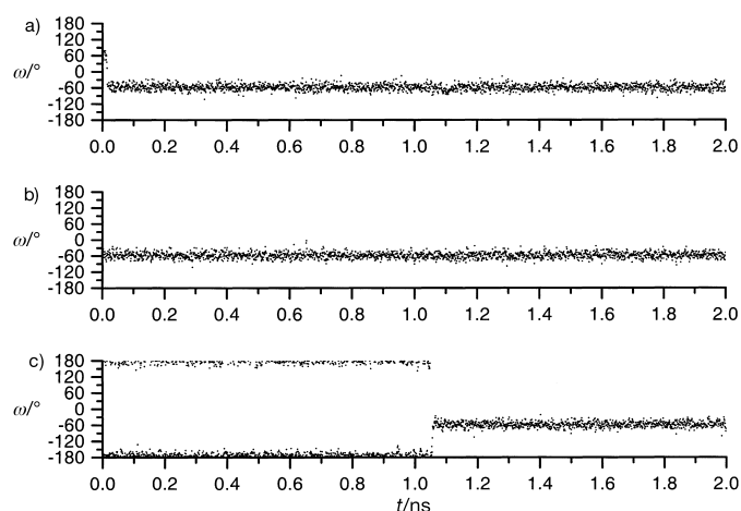
Figure 1. Trajectory plots for 4- \text{Man}\alpha(1 \rightarrow 6)3\text{-Man} linkage, \omega torsion angle of the MD simulations of compound 1a for a) tg , b) gt and c) gg starting structures.
