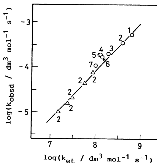
Fig. 1. Comparison of the rate constants k obsd of acid-catalyzed reduction of ketones by unprotonated AcrH 2 in the absence (o) and the presence of added water (Δ) in MeCN containing 2.0 mol dm -3 HClO 4 at 331 K with the corresponding rate constants k et of photoinduced electron transfer from [Ru(bpy) 3 ] 2+* to the ketones at 298 K. The numbers refer to the ketones in Table 1.
