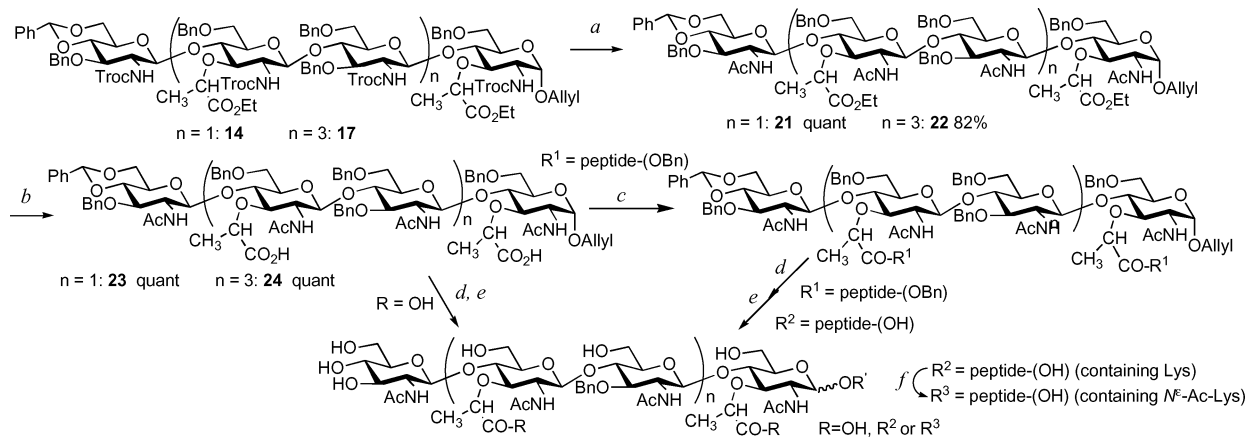
Scheme 4 Synthesis of tetrasaccharide and octasaccharide peptides: (a) \text{Zn-Cu} , \text{AcOH} then \text{Ac}_2\text{O} , \text{Py} ; (b) \text{LiOH} , Dioxane, THF, \text{H}_2\text{O} ; (c) appropriate peptide \text{HCl} salt, \text{WSCl}\cdot\text{HCl} , \text{HOBt} , \text{TEA} , \text{CH}_2\text{Cl}_2 ; (d) Ir complex, \text{H}_2 , THF, then \text{I}_2 , \text{H}_2\text{O} ; (e) \text{Pd}(\text{OH})_2 , \text{AcOH} , \text{H}_2 (10 \text{kg cm}^{-2} ); (f) \text{Ac}_2\text{O} , \text{TEA} , \text{MeOH} .
