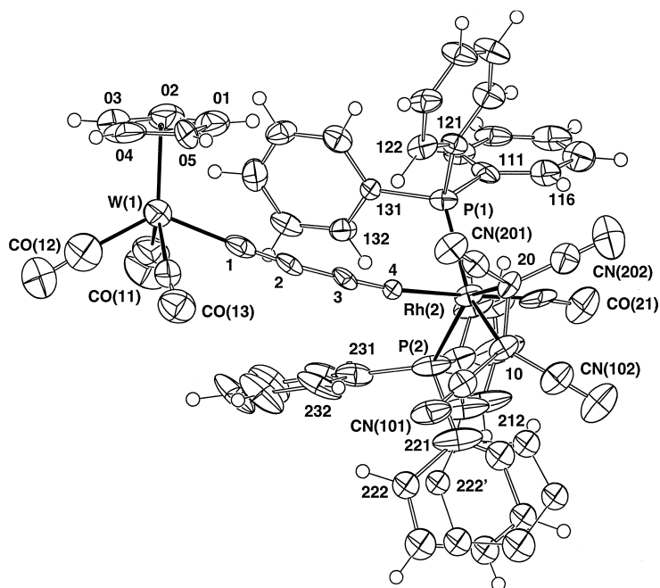
Fig. 1. Plot of a molecule of \{\text{Cp}(\text{OC})_3\text{W}\}\text{C}\equiv\text{CC}\{\text{Rh}(\text{CO})[\eta\text{-C}_2(\text{CN})_4]\}(\text{PPh}_3)_2 ( 5 ), showing atom numbering scheme. In this and subsequent figures, non-hydrogen atoms are shown as 20% thermal ellipsoids; hydrogen atoms have arbitrary radii of 0.1 Å.
