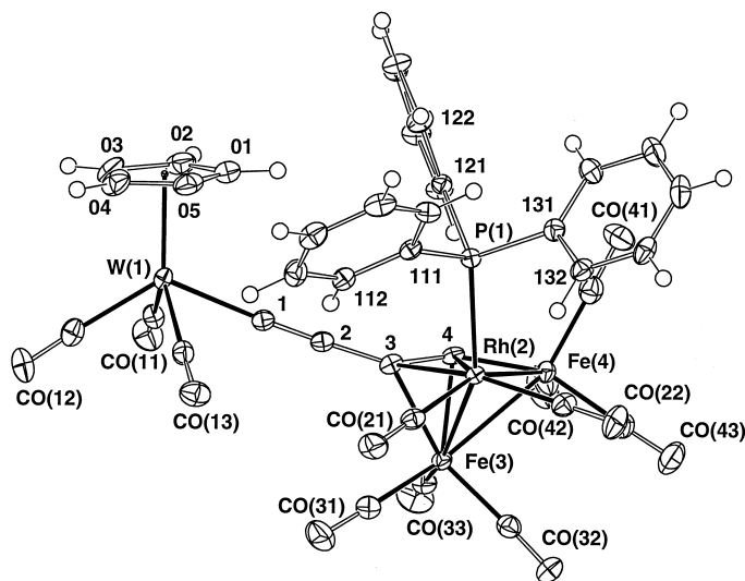
Fig. 2. Plot of a molecule of {Cp(OC) 3 W}C≡CC 2 {Fe 2 Rh(CO) 8 (PPh 3 )} ( 7 ), showing atom numbering scheme.
