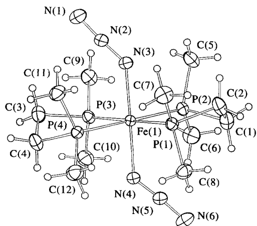
Fig. 1. View of the complex trans - \text{Fe(N}_3)_2(\text{dmpe})_2 ( 2a ) showing atom labelling.
