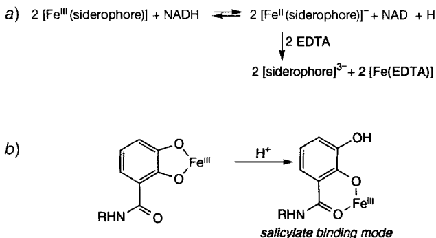
Scheme 1. Possible Release Mechanism for Iron Siderophores: a) Reduction by NADH; b) Protonation
