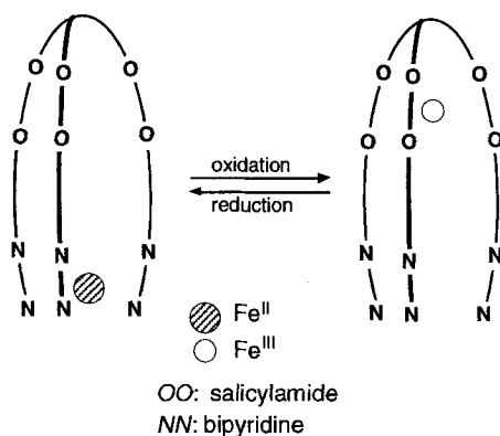
Scheme 2. An Iron-Based Molecular Switch
