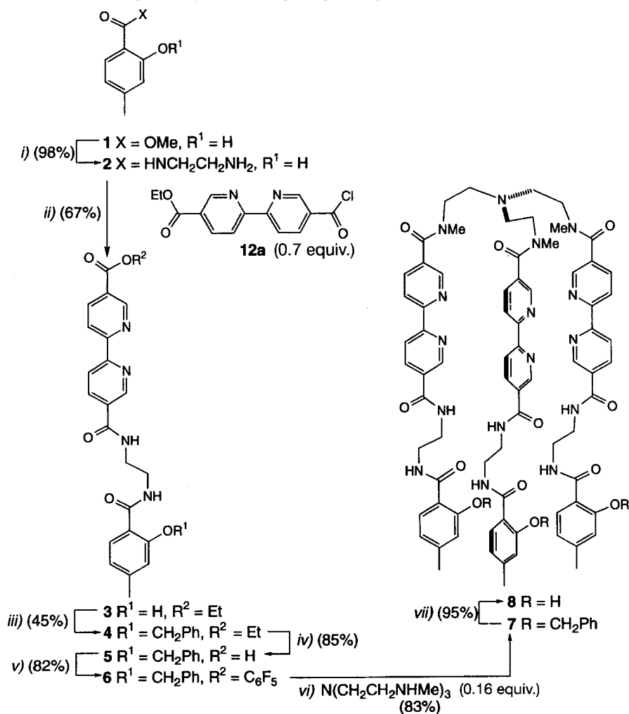
Scheme 4. Preparation of the NN -Merged Tripodal Ligand 8 via the Single-Strand Route
