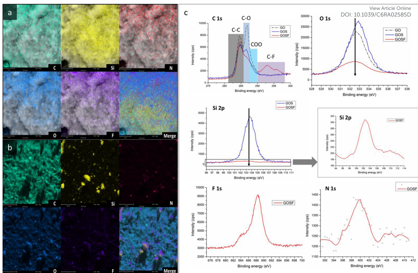
Figure 7. Surface analysis of GOSF. (a-b): EDX mapping performed in two different zones of GOSF characterized by higher (a), and lower content of silica (b); the scale bar for the mapped zone of panel (a) and (b) are respectively 3 μm and 30 μm. (c): XPS results of GOSF with C1s and O1s spectra of GO and GOS, and Si2p spectrum of GOS for comparison.
