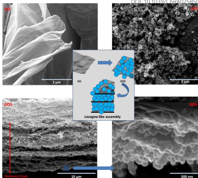
Figure 5. SEM micrographs of a GO lamella before (top left) and after (top right) silica-decoration, morphology of lasagna-like self-assembled films at different magnification (bottom)
