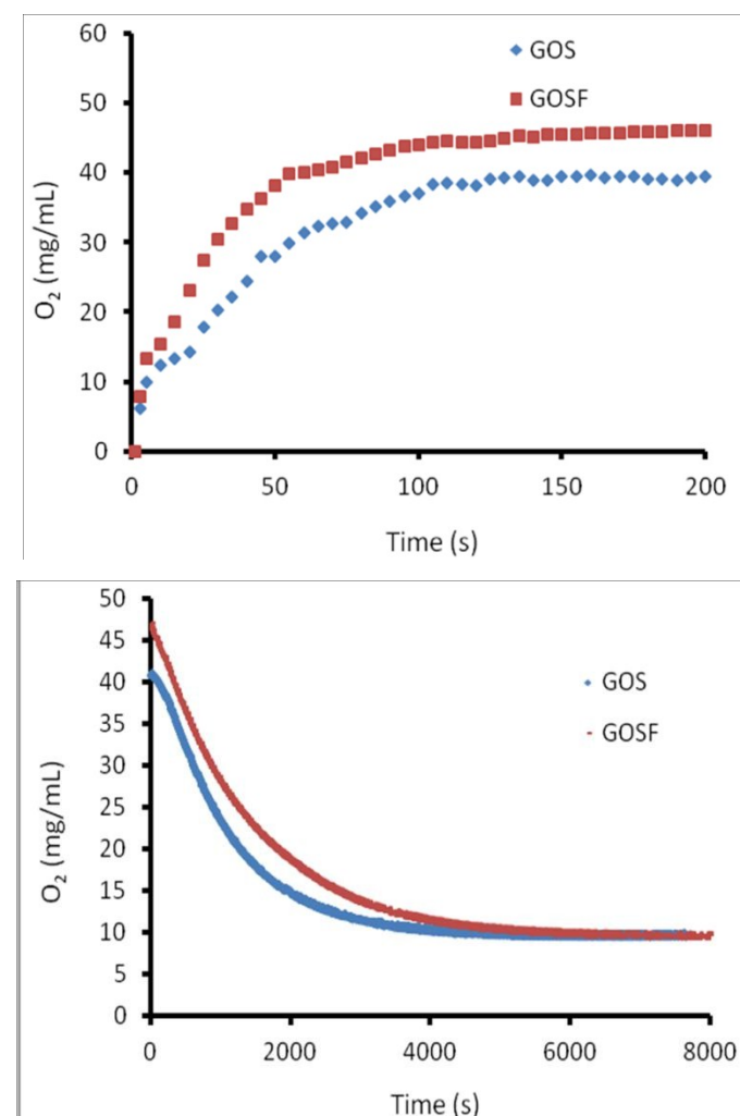
Figure 8. Oxygen uptake (top) and release (bottom) curves from aqueous solutions containing composites at 25°C
