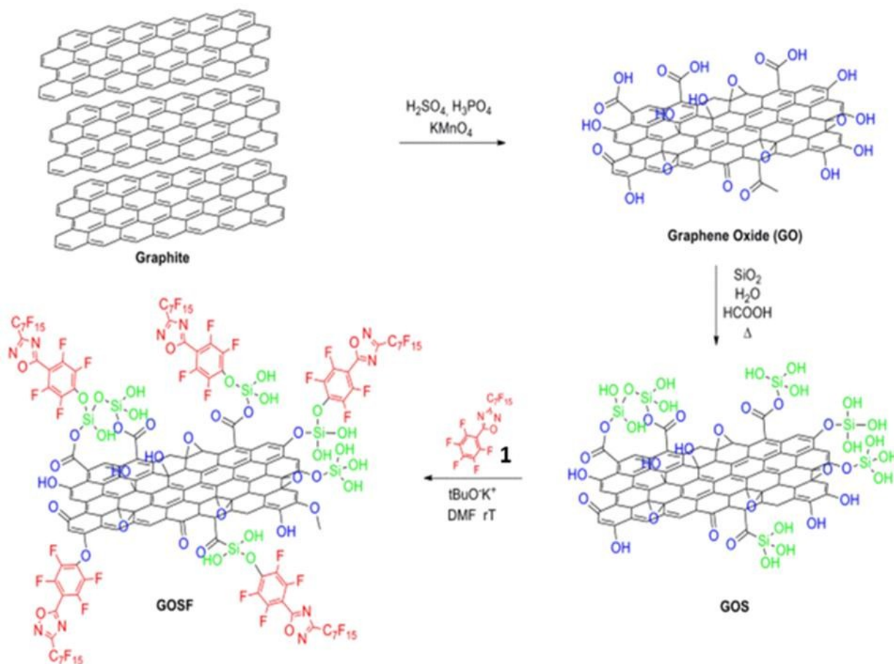
Figure 1. Route to GOSF: GO was synthesized via the modified Hummers method, 13 and silica-GO (GOS) composite was prepared by Fischer esterification in water and 2% of HCOOH at 120\text{ }^{\circ}\text{C} between the -\text{COOH} and epoxy groups of GO and the -\text{OH} moieties of the silica. The functionalization with fluorinated tails has been realized by aromatic nucleophilic substitution. In particular, a 3-pentadecafluoroheptyl, 5-perfluorophenyl-1,2,4-oxadiazole ( 1 ), has been introduced very easily by nucleophilic substitution operated by the oxygenated functionalities present on the surface of the GO-silica nanohybrid
