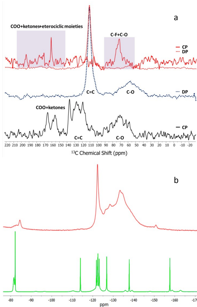
Figure 4. a) 13 C { 1 H} MAS NMR spectra of GO (black), GOS (blue) and GOSF (red) registered in direct (DP) and/or cross polarization (CP) (dotted line); b) 19 F MAS NMR spectra of GOSF (red) and 1 (green).
