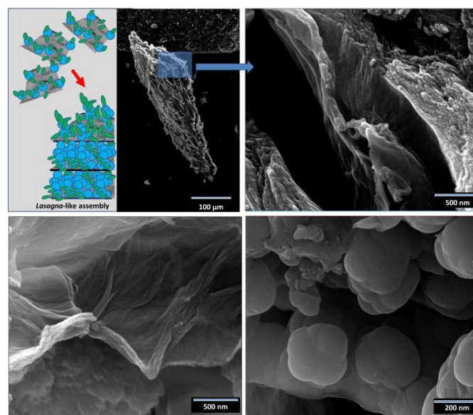
Figure 6. SEM analysis of GOSF SEM analysis of a GOSF device with detailed micrographs of its hierarchical structure at different magnifications, and a detailed picture of a fluorinated zone not covered by silica (bottom left).
