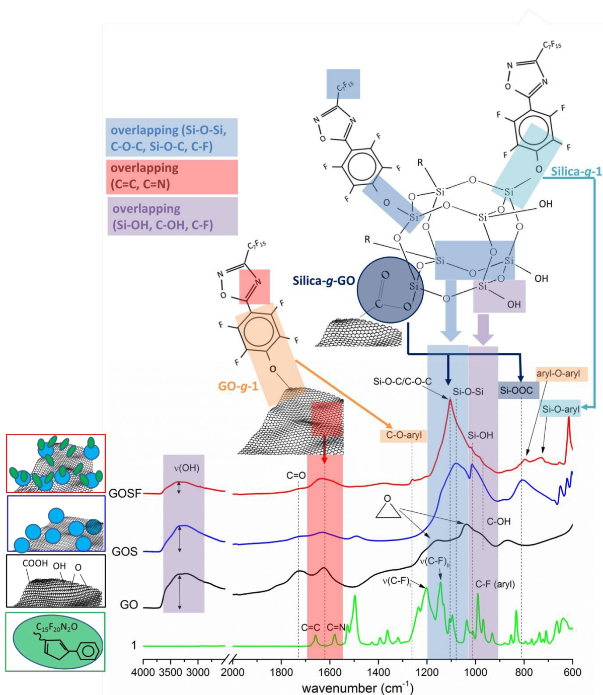
Figure 2. FTIR spectra of 1 (green), GOS (blue), GOSF (red).
