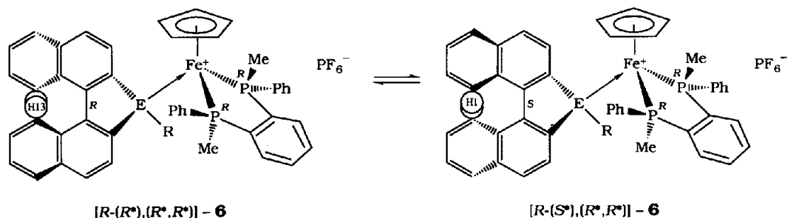
Fig. 5. Interconversion of diastereomers [(\text{R}^*), (\text{R}^*, \text{R}^*)]\text{-6} and [(\text{S}^*), (\text{R}^*, \text{R}^*)]\text{-6} .
