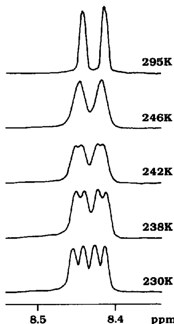
Fig. 4. Variable temperature ^1\text{H} NMR data for \text{H}_1 and \text{H}_{13} of (\pm) -3 ( \text{R} = \text{Me} ) in dichloromethane- d_2 .
