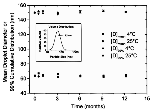
Fig. 1. Mean droplet diameter, [D]_{\text{mean}} , and 99% cumulative distribution, [D]_{99\%} , of QW8184 as a function of storage time and temperature. This particular lot of QW8184 (lot A) incorporated 9.0 mg/mL paclitaxel and was stored at 4°C or 25°C. The actual volume-weighted particle size distribution of QW8184 is shown in the insert with a mean droplet diameter of 62 nm.
