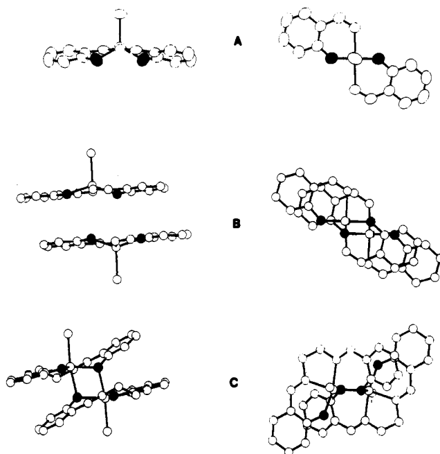
Figure 3. Molecular structures of (A) the monomeric form of Fe(SANE) 2 Cl, (B) the dimeric form of Fe(SANE) 2 Cl, 1 and (C) the dimeric form of Fe(Salen)Cl. 2 In structures A and B, the phenylethyl groups have been omitted for clarity. All hydrogen atoms have been omitted. The oxygen atoms in these drawings are black.
