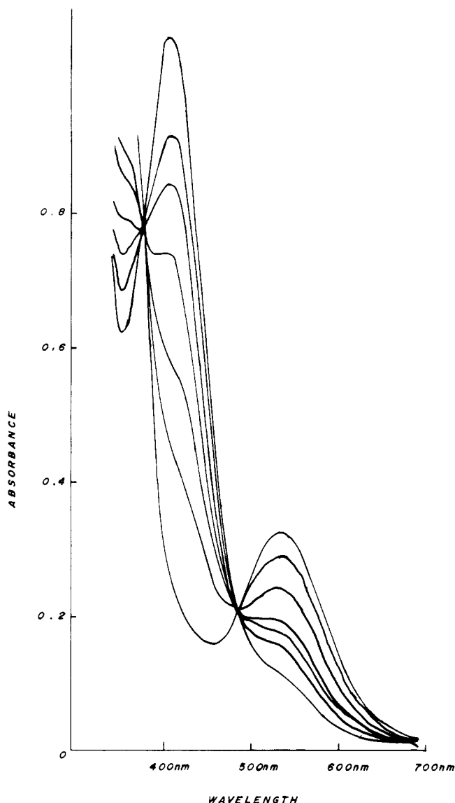
Figure 1. Spectral changes for the reaction \text{Fe(14ane)(CH}_3\text{CN)(CO)}^{2+} + \text{CH}_3\text{CN} \rightarrow \text{Fe(14ane)(CH}_3\text{CN)}_2^{2+} + \text{CO} in acetonitrile 25 °C. Spectra for decreasing absorbance at 420 nm are recorded at times 0, 3.5, 7.5, 12, 20.5, 39, and 67 min.
