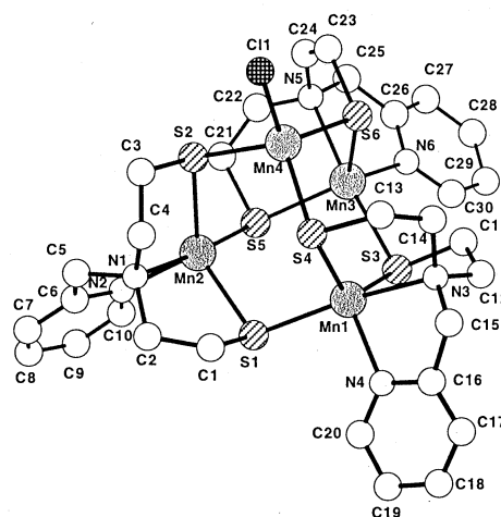
Figure 1. Perspective view of complex cation of 1 , showing the atom-labeling scheme. Selected bond distances ( d /Å) and angles ( φ /°): Mn1-Mn2 4.033(3), Mn1-Mn3 4.025(2), Mn1-Mn4 3.954(2), Mn2-Mn3 4.031(2), Mn2-Mn4 3.992(3), Mn3-Mn4 4.000(2), Mn1-S1 2.496(4), Mn1-S3 2.461(3), Mn1-S4 2.468(3), Mn1-N3 2.31(1), Mn1-N4 2.200(9), Mn2-S1 2.452(4), Mn2-S2 2.465(3), Mn2-S5 2.503(3), Mn2-N1 2.324(8), Mn2-N2 2.19(1), Mn3-S3 2.498(3), Mn3-S5 2.460(4), Mn3-S6 2.491(4), Mn3-N5 2.307(9), Mn3-N6 2.213(8), Mn4-Cl1 2.307(4), Mn4-S2 2.453(4), Mn4-S4 2.454(3), Mn4-S6 2.447(3); S1-Mn1-S3 101.6(1), S1-Mn1-S4 99.0(1), S1-Mn1-N3 172.5(2), S1-Mn1-N4 97.9(3), S3-Mn1-S4 125.6(1), S3-Mn1-N3 83.7(2), S3-Mn1-N4 110.6(3), S4-Mn1-N3 81.8(3), S4-Mn1-N4 115.5(3), N3-Mn1-N4 75.2(4), S1-Mn2-S2 123.6(1), S1-Mn2-S5 102.3(1), S1-Mn2-N1 83.6(2), S1-Mn2-N2 105.9(2), S2-Mn2-S5 97.9(1), S2-Mn2-N1 81.1(2), S2-Mn2-N2 121.3(3), S5-Mn2-N1 173.4(3), S5-Mn2-N2 100.4(2), N1-Mn2-N2 74.8(3), S3-Mn3-S5 101.1(1), S3-Mn3-S6 99.3(1), S3-Mn3-N5 173.8(3), S3-Mn3-N6 98.7(3), S5-Mn3-S6 124.3(1), S5-Mn3-N5 82.9(3), S5-Mn3-N6 112.0(3), S6-Mn3-N5 82.1(3), S6-Mn3-N6 115.3(3), N5-Mn3-N6 75.4(3), Cl1-Mn4-S2 104.2(2), Cl1-Mn4-S4 111.1(1), Cl1-Mn4-S6 115.2(1), S2-Mn4-S4 110.5(1), S2-Mn4-S6 106.7(1), S4-Mn4-S6 108.9(1).
