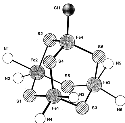
Figure 2. Perspective view of coordination spheres of cation of 2 . Selected bond distances ( \text{\AA} ) and angles ( ^\circ ): Fe1-Fe 3.967(2), Fe1-Fe3 3.962(3), Fe1-Fe4 3.826(2), Fe2-Fe3 3.960(3), Fe2-Fe4 3.860(3), Fe3-Fe4 3.888(3), Fe1-S1 2.399(5), Fe1-S3 2.362(5), Fe1-S4 2.381(4), Fe1-N3 2.26(1), Fe1-N4 2.13(1), Fe2-S1 2.342(3), Fe2-S2 2.381(4), Fe2-S5 2.412(5), Fe2-N1 2.28(1), Fe2-N2 2.13(1), Fe3-S3 2.405(4), Fe3-S5 2.365(5), Fe3-S6 2.401(5), Fe3-N5 2.275(9), Fe3-N6 2.14(1), Fe4-Cl1 2.256(4), Fe4-S2 2.385(4), Fe4-S4 2.357(4), Fe4-S6 2.370(5), S1-Fe1-S3 100.4(2), S1-Fe1-S4 97.2(2), S1-Fe1-N3 173.7(4), S1-Fe1-N4 97.3(4), S3-Fe1-S4 123.3(2), S3-Fe1-N3 84.3(4), S3-Fe1-N4 111.7(4), S4-Fe1-N3 83.4(3), S4-Fe1-N4 118.8(4), N3-Fe1-N4 77.0(5), S1-Fe2-S2 121.7(1), S1-Fe2-S5 100.2(1), S1-Fe2-N1 84.1(2), S1-Fe2-N2 108.1(3), S2-Fe2-S5 97.5(2), S2-Fe2-N1 82.5(3), S2-Fe2-N2 123.0(2), S5-Fe2-N1 174.8(3), S5-Fe2-N2 99.1(4), N1-Fe2-N2 76.7(5), S3-Fe3-S5 99.5(2), S3-Fe3-S6 97.1(1), S3-Fe3-N5 175.3(4), S3-Fe3-N6 98.5(3), S5-Fe3-S6 122.7(2), S5-Fe3-N5 84.0(4), S5-Fe3-N6 113.5(4), S6-Fe3-N5 83.5(4), S6-Fe3-N6 117.6(4), N5-Fe3-N6 77.1(4), Cl1-Fe4-S2 104.2(1), Cl1-Fe4-S4 110.8(2), Cl1-Fe4-S6 114.7(2), S2-Fe4-S4 111.3(2), S2-Fe4-S6 106.7(2), S4-Fe4-S6 109.0(1).
