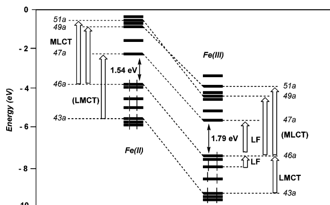
Figure 5. Orbital diagram for [(\text{H}_3\text{P})_2(\eta^5\text{-C}_5\text{H}_5)\text{Fe}(\text{C}\equiv\text{C})\text{-1,4-(C}_6\text{H}_4)\text{NH}_2]^{0+} ( 1j-H / 1j-H + ) showing the effect of oxidation on the energy levels. The arrows indicate the possible excitations leading to MLCT, LMCT, or LF transitions in the visible range. Transitions in parentheses were not observed in the visible spectrum (400–800 nm).
