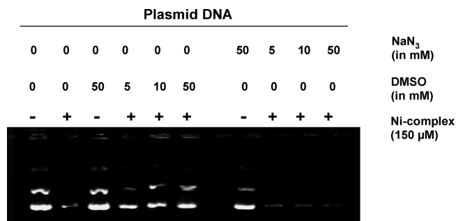
Figure 9. Lane 1: pGEM3Z plasmid DNA (200 ng in base pair). Lane 2: pGEM3Z plasmid DNA (200 ng in base pair) with 150 μM of the complex 1 alone. Lanes 4–6: pGEM3Z plasmid DNA (200 ng in base pair) with 150 μM of the complex 1 in the presence of radical scavenger DMSO. Lanes 8–10: pGEM3Z plasmid DNA (200 ng in base pair) with 150 μM of the complex 1 in the presence of NaN 3 . The pGEM3Z plasmid DNA was also incubated with DMSO (lane3) and NaN 3 (lane7) alone to show that these scavengers do not have any effect on the DNA.
