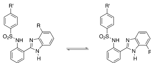
Scheme 3. Nondegenerate prototropic equilibrium of the tautomer pairs of the substituted ligands 7a/b–9a/b .
