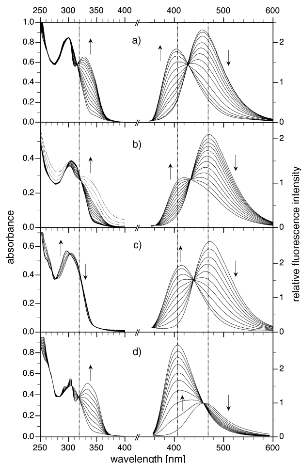
Figure 5. UV-visible absorbance (left) and fluorescence emission spectra (right) of ligands a) 6b , b) 7b , c) 8b , and d) 9b as a function of added \text{Zn}^{\text{II}} (excitation at the isosbestic point of the UV-visible traces, pH 7.20, 10 mM PIPES, 0.1 M \text{KClO}_4 ).
