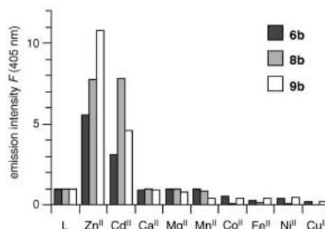
Figure 7. Emission intensity at 405 nm ( \lambda_{\text{ex}} = 320 nm) of ligands 6b , 8b , and 9b in response to various metal cations. Concentrations: 6b 10 \mu\text{M} , all \text{M}^{2+} 1 mM; 8b 10 \mu\text{M} , \text{Ca}^{\text{II}} , \text{Mg}^{\text{II}} 1 mM, all other \text{M}^{2+} 10 \mu\text{M} ; 9b 10 \mu\text{M} , \text{Ca}^{\text{II}} , \text{Mg}^{\text{II}} 1 mM, all other \text{M}^{2+} 10 \mu\text{M} (pH 7.2, 10 mM PIPES, 0.1 M \text{KClO}_4 ).
