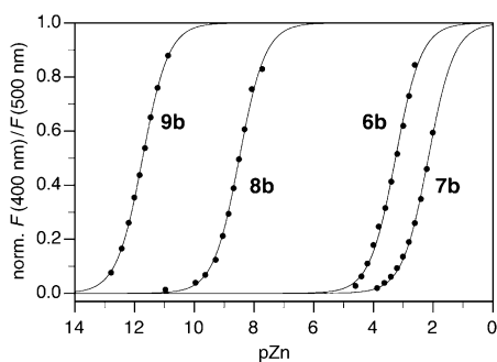
Figure 6. Change of the emission intensity ratio at 400 and 500 nm ( \lambda_{\text{ex}} = 320 nm) for ligands 6b–9b as a function of free \text{Zn}^{\text{II}} ( \text{pZn} = -\log[\text{Zn}^{\text{II}}_{\text{free}}] , pH 7.2, 10 mM PIPES, 0.1 M \text{KClO}_4 ).
