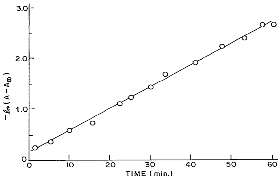
Fig. 1. A typical plot of infrared spectroscopic data for the cleavage of \eta^5\text{-C}_5\text{H}_5\text{Fe(CO)}_2\text{CH}_3 by a tenfold excess of \text{CF}_3\text{CO}_2\text{H} in \text{CH}_2\text{Cl}_2 at 25^\circ\text{C} .
