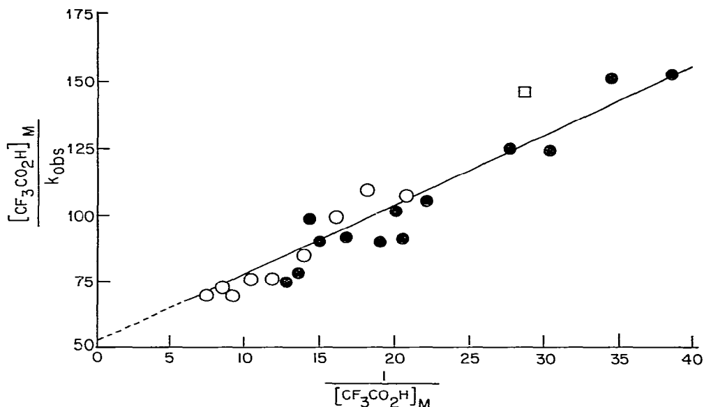
Fig. 4. Cleavage of \eta^5\text{-C}_5\text{H}_5\text{Fe(CO)}_2\text{CH}_3 by a tenfold excess of \text{CF}_3\text{CO}_2\text{H} in \text{CH}_2\text{Cl}_2 at 25^\circ\text{C} . The data are those used in Figure 2.
