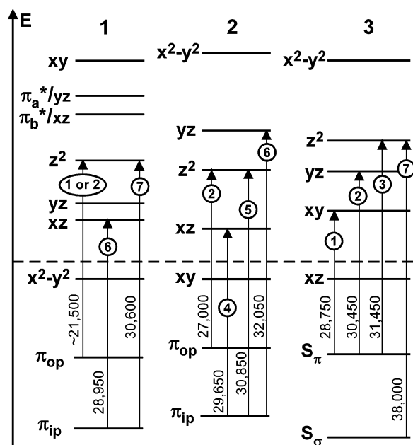
Figure 11. Energy-level diagram displaying the experimentally determined transition energies (in \text{cm}^{-1} ) within the MO framework provided by DFT calculations for 1–3. Transitions are labeled according to the numbering scheme used in Figure 4 and Table 2.
