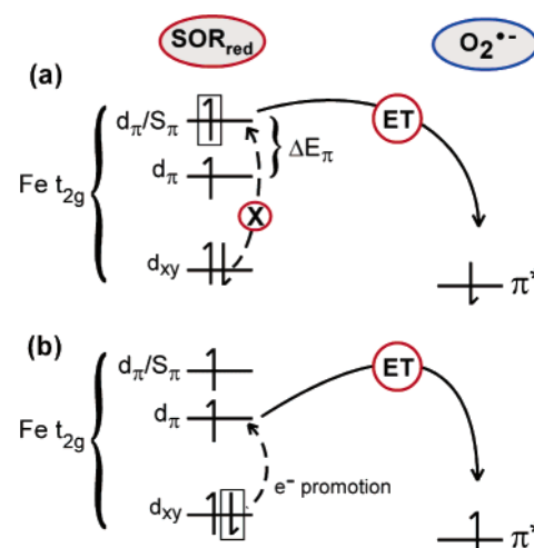
Figure 12. Two possible scenarios for inner-sphere electron transfer (ET) from the Fe(II) center of SOR to the superoxide radical (O 2 •− ). (a) The “boxed” electron in the Fe d π /S π orbital is transferred to the \pi^* acceptor orbital of O 2 •− , yielding an Fe(III) S = 3/2 intermediate. (b) Orbital mixing “promotes” the boxed electron from the d xy orbital to the nearby d π orbital, followed by ET to O 2 •− . This mechanism directly results in the S = 5/2 state of the oxidized enzyme.
