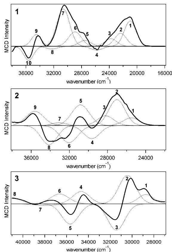
Figure 4. Gaussian-resolved (····) solid-state MCD spectra (—) of complexes 1–3 . Spectra were obtained with a magnetic field of 7 T at a temperature of 4 K for 1 and 2 and 20 K for 3 . Band energies and parameters are summarized in Table 2. Note that each spectrum is plotted over a different energy range (x-axes are not the same for 1–3 ).
