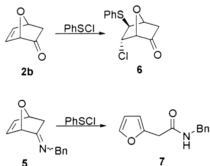
Scheme 1
