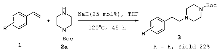
Scheme 2. Base-catalyzed hydroamination of aryl olefins with N -Boc-piperazine.
