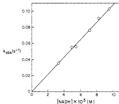
Figure 1. Plot of the observed pseudo-first-order rate constants vs. NADH concentration. [\text{NaClO}_4] = 0.1 \text{ M} .
