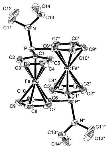
Figure 2. ORTEP drawing of anti - 3 with 50% thermal ellipsoids. Hydrogen atoms are omitted for clarity. Selected bond distances (Å) and angles (deg): P–N 1.694(2), P–C(1) 1.814(2), P–C(6*) 1.831(2), N–P–C(1) 100.75(10), N–P–C(6*) 101.53(9), C(1)–P–C(6*) 106.04(9). Symmetry transformation used to generate equivalent (asterisked) atoms: (– x + 1.5, – y + 0.5, – z ).
