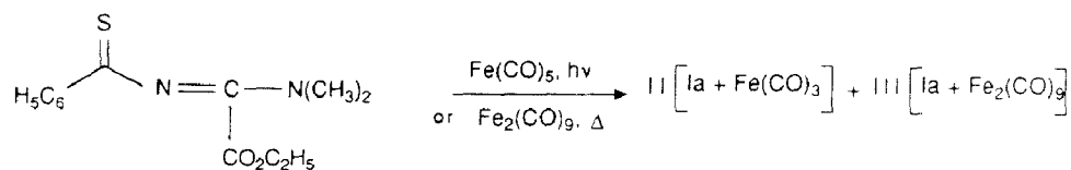
Ia Scheme 1
