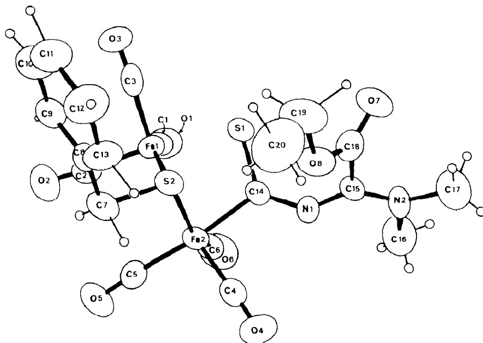
Fig. 3. Structure of compound IV.
