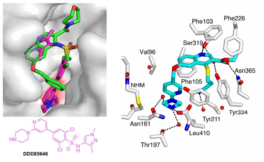
Fig. 4 (Left) View of 19 (green carbons) in LmNMT in cylinder format. The surface of LmNMT is shown in grey. 19 is superimposed with DDD85646 (2,6-dichloro-4-(2-piperazin-1-ylpyridin-4-yl)-N-(1,3,5-trimethyl-1H-pyrazol-4-yl)-benzenesulfonamide; magenta carbons), a known NMT inhibitor. The surface above the C-terminal leucine of NMT is colored in red. (Right) Crystal structure of 26 (cyan carbons) in complex with PvNMT and non-hydrolyzable MyrCoA (pdb accession code: 5G22). Selected side chains of PvNMT are shown in cylinder (format) and labeled according to PvNMT numbering. Dashed lines indicate electrostatic/H-bond interactions. For further views of 26 in complex with PvNMT and LmNMT, see Supplementary Figs. S4, S5 & S6.
