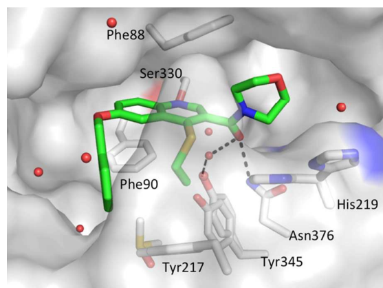
Figure 3. Structure of quinoline 19 in a ternary complex with LmNMT and MyrCoA (PDB accession code: 5G20). 19 is shown in cylinder format and colored by atom: carbon (green), oxygen (red), nitrogen (blue) and sulphur (yellow). A transparent LmNMT surface is shown in grey. The side chains of selected LmNMT residues located within 4 Å of 19 are displayed as grey sticks, and labeled. Water molecules are shown as red spheres. Polar interactions with LmNMT and solvent are represented as black dashed lines. For a stereo view, see Supplementary Fig. S2.
