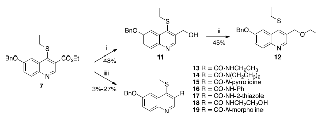
Scheme 3 Syntheses of alcohol, ether and amide derivatives 11–19 . Reagents and conditions: (i) \text{LiAlH}_4 , THF, 0 °C, 1 h; (ii) t\text{BuOK} , DMSO, RT then EtI, 60 °C, 1 h; (iii) \text{AlMe}_3 , amine, toluene, -15 °C then 7 , RT, 24 h
