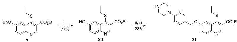
Scheme 4 Synthesis of compound 21 . Reagents and conditions: (i) methanesulfonic acid 10% (v/v) in TFA, 60 °C, 4 h; (ii) 6-(4-Boc-piperazin-1-yl)pyridin-3-yl)methanol, DEAD, PPh 3 , THF, RT, 16 h; (iii) TFA 20% in DCM, RT, 40 min.
