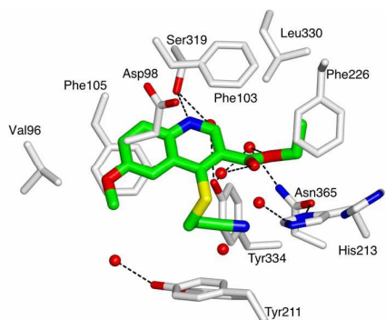
Fig. 2 Structure of quinoline 1 in a ternary complex with P. vivax NMT and S-(2-oxo)pentadecylCoA (NHM) (PDB accession code: 5G1Z). View of 1 in chain A of PvNMT in cylinder format and colored by atom: carbon (green), oxygen (red), nitrogen (blue), sulphur (yellow). The side chains of residues located within 4 Å of 1 are displayed as cylinders and labelled. Water molecules are shown as red spheres. Polar interactions with PvNMT are represented as dashed lines. Y211 and H213 are shown in two alternate conformations. For a stereoview, see Supplementary Fig. S2.
