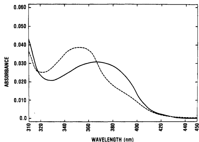
Figure 2. Pteridine spectral shift upon binding to L. casei DHFR. The spectrum (solid curve) of 4 \mu M 2'-fluoroaminopterin was obtained in 0.05 M potassium phosphate buffer, pH 7.0, containing 0.5 M KCl. Addition of a small aliquot (25 \mu L) of enzyme solution to a final concentration of 5 \mu M in both the sample and reference cuvette gives the dashed curve spectrum.
