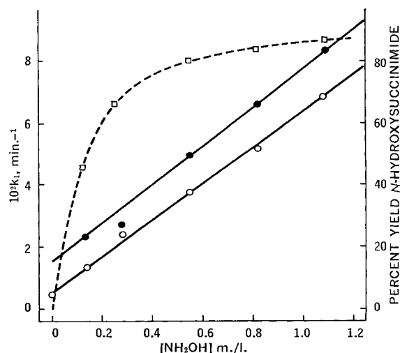
Figure 5 —Pseudo first-order rate constants, k_1 (left ordinate), as a function of [NH 2 OH] for 0.016 M succinimide at 40°, pH 9.50 (○) and pH 10.5 (●). The percent yield of N -hydroxysuccinimide (right ordinate, □) as a function of [NH 2 OH] at 40°, pH 9.50.
