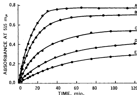
Figure 1 —Increase in absorbance at 515 mμ as a function of reaction time due to the formation of the hydroxamic acid-iron complex formed by dilution of aliquots from reactions containing 0.016 M succinimide and [NH 2 OH] equal to: A, 1.09 M; B, 0.82; C, 0.55; D, 0.28; and E, 0.14 at pH 10.50, 40.0°.
