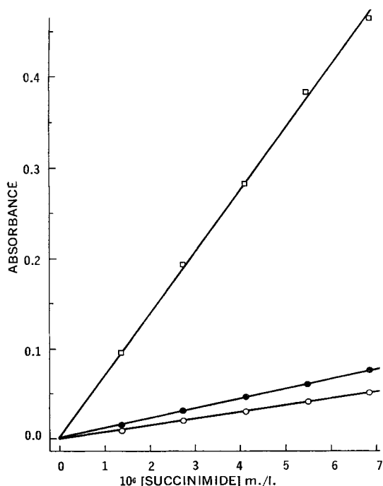
Figure 6 —Comparison of assay methods for succinimide by reacting with \text{NH}_2\text{OH} at 40^\circ , pH 8.3 and measuring the N -hydroxysuccinimide at 260\text{ m}\mu (□) or the hydroxamic acid-iron complex at 515\text{ m}\mu (○) and at pH 11.7 measuring the iron complex at 515\text{ m}\mu (●).
