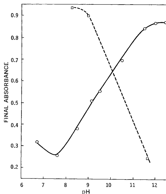
Figure 4 —The final absorbance values at 515 m \mu due to formation of the hydroxamic acid-iron complex (○) and the final absorbance values at 260 m \mu due to formation of N -hydroxysuccinimide (□) from reactions containing fixed concentrations of succinimide and NH 2 OH and varying pH at 40°.
