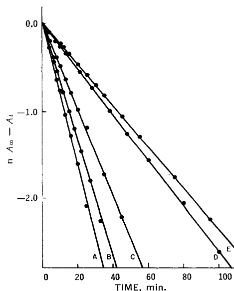
Figure 2 —First-order plots for the increase in absorbance at 515 m\mu due to the hydroxamic acid-iron complex formed from aliquots of reactions containing 0.016 M succinimide and [NH 2 OH] equal to A, 1.09 M ; B, 0.82; C, 9.55; D, 0.28; and E, 0.14 at pH 10.50, 40°.
