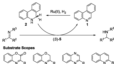
Scheme 2. Biomimetic Asymmetric Hydrogenation Promoted by Dihydrophenanthridine
